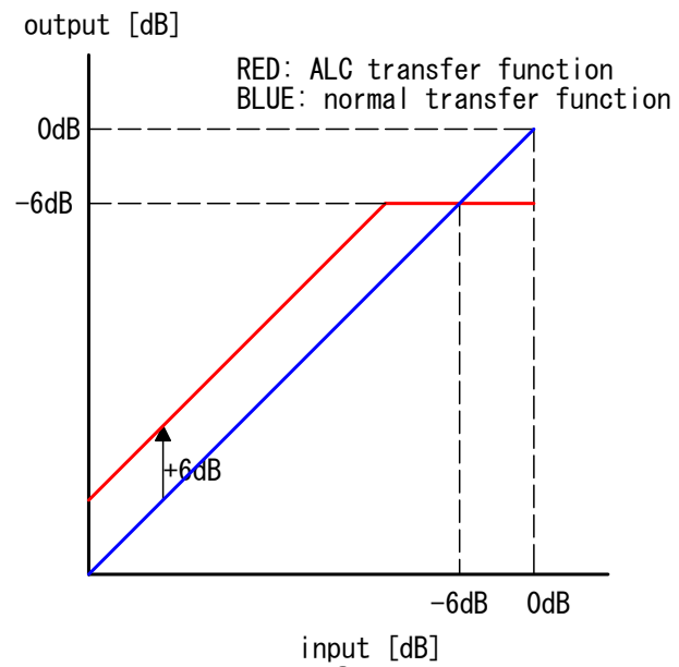
ALC transfer curve
