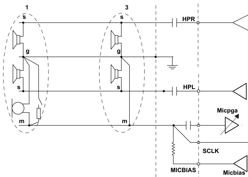
Figure 5-58. Jack Connections for Headset Detection
