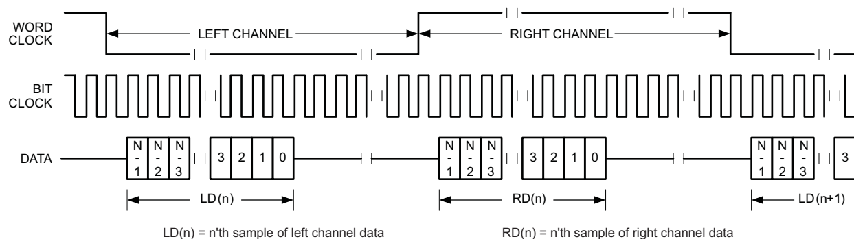
Figure 5-49. Timing Diagram for I²S Mode with offset=0 and bit clock invert
