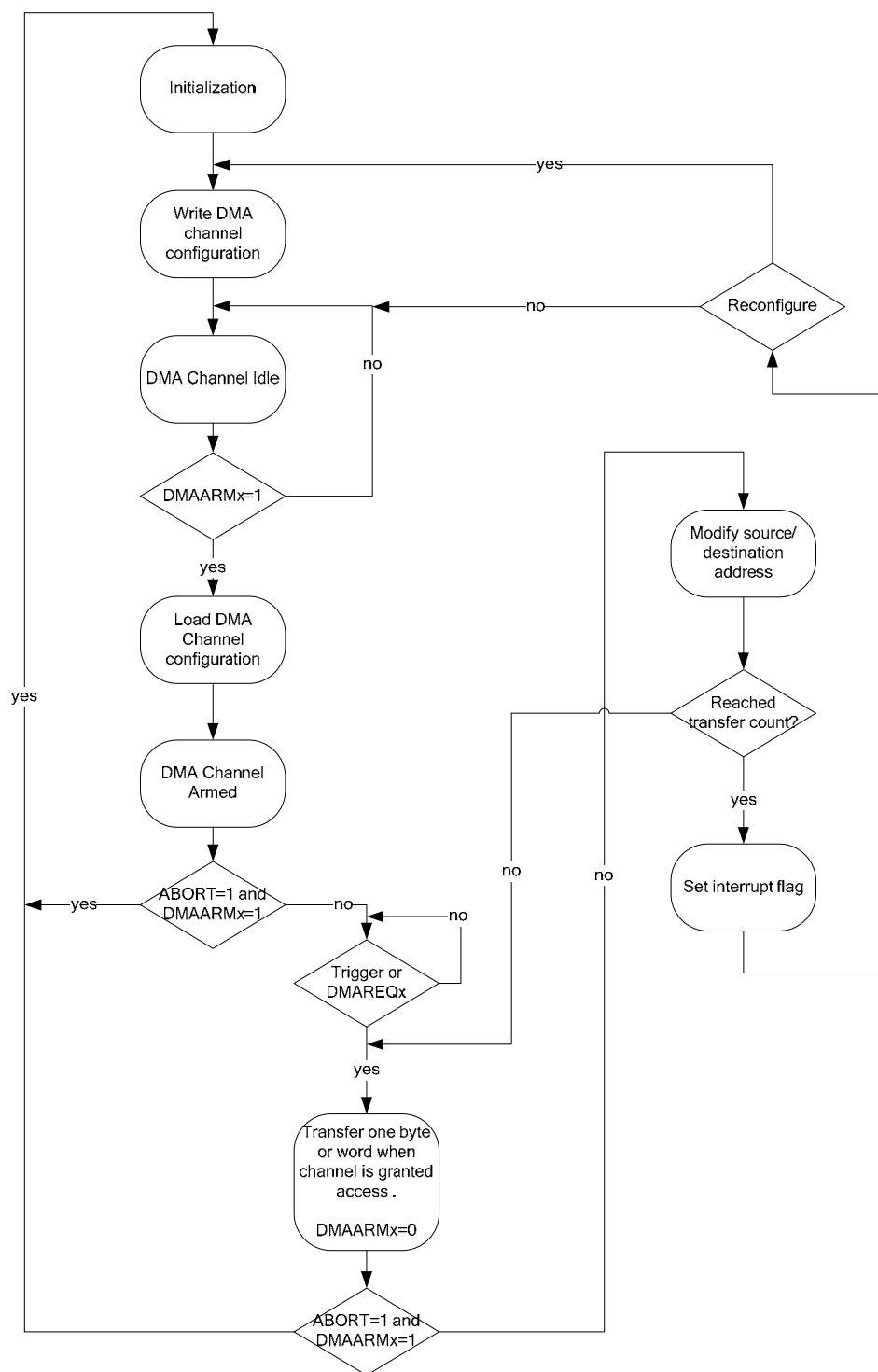
Figure 18: DMA Operation
