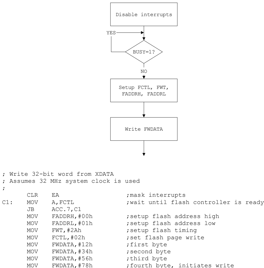
Figure 35: Flash write performed from XDATA
