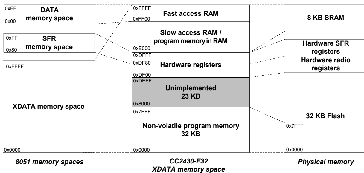
Figure 7: CC2430-F32 XDATA memory space
