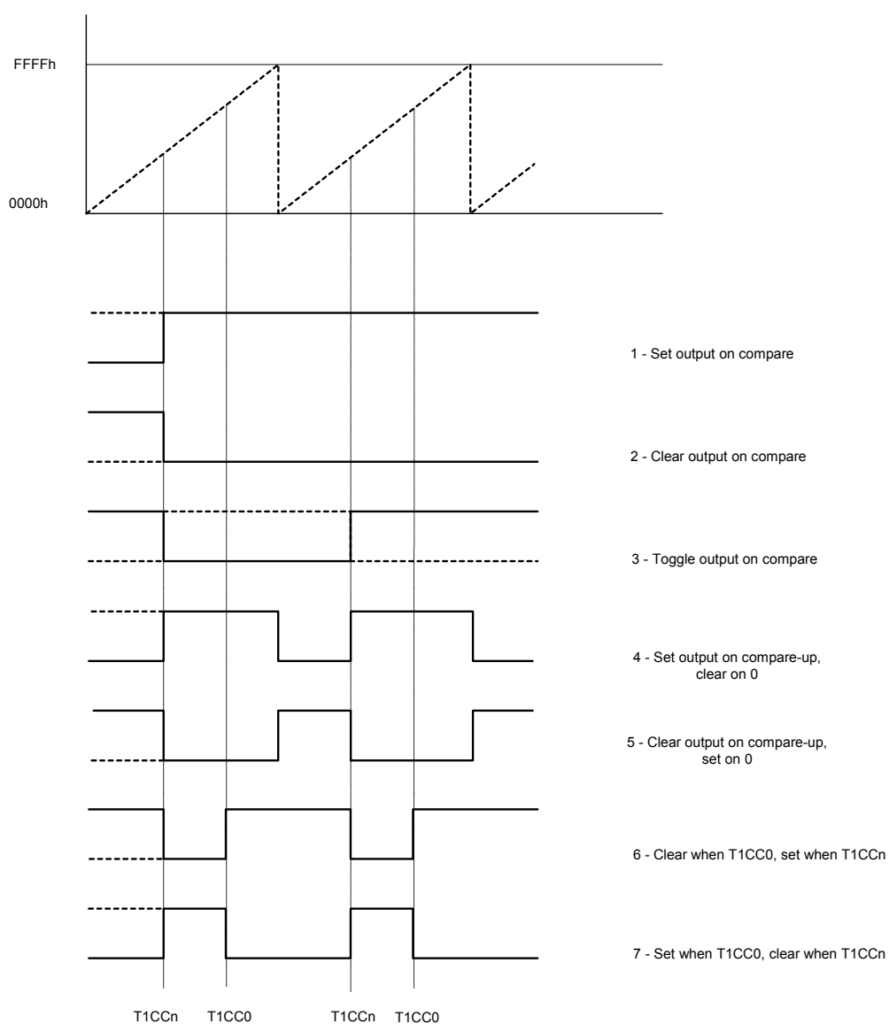
Figure 23: Output compare modes, timer free-running mode
