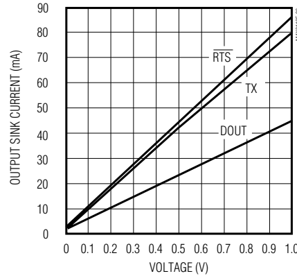
MAX3110E TX, \overline{\text{RTS}} , DOUT OUTPUT CURRENT vs. OUTPUT LOW VOLTAGE ( V_{CC} = +5\text{V} )
