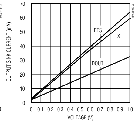
MAX3111E TX, \overline{\text{RTS}} , DOUT OUTPUT CURRENT vs. OUTPUT LOW VOLTAGE ( V_{CC} = +3.3\text{V} )
