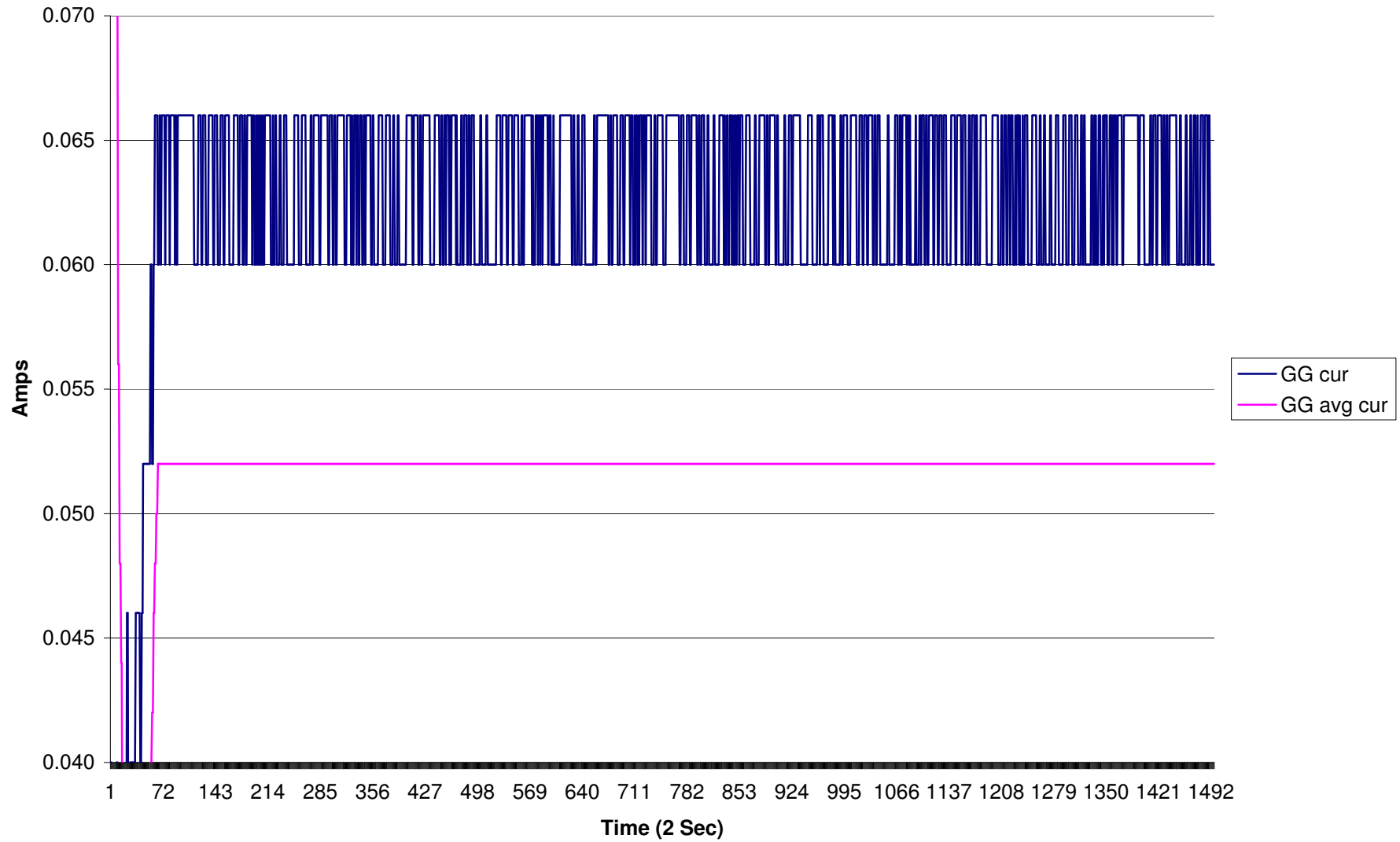
NiMH Maintenance current cal'ed to GG AVG Current
