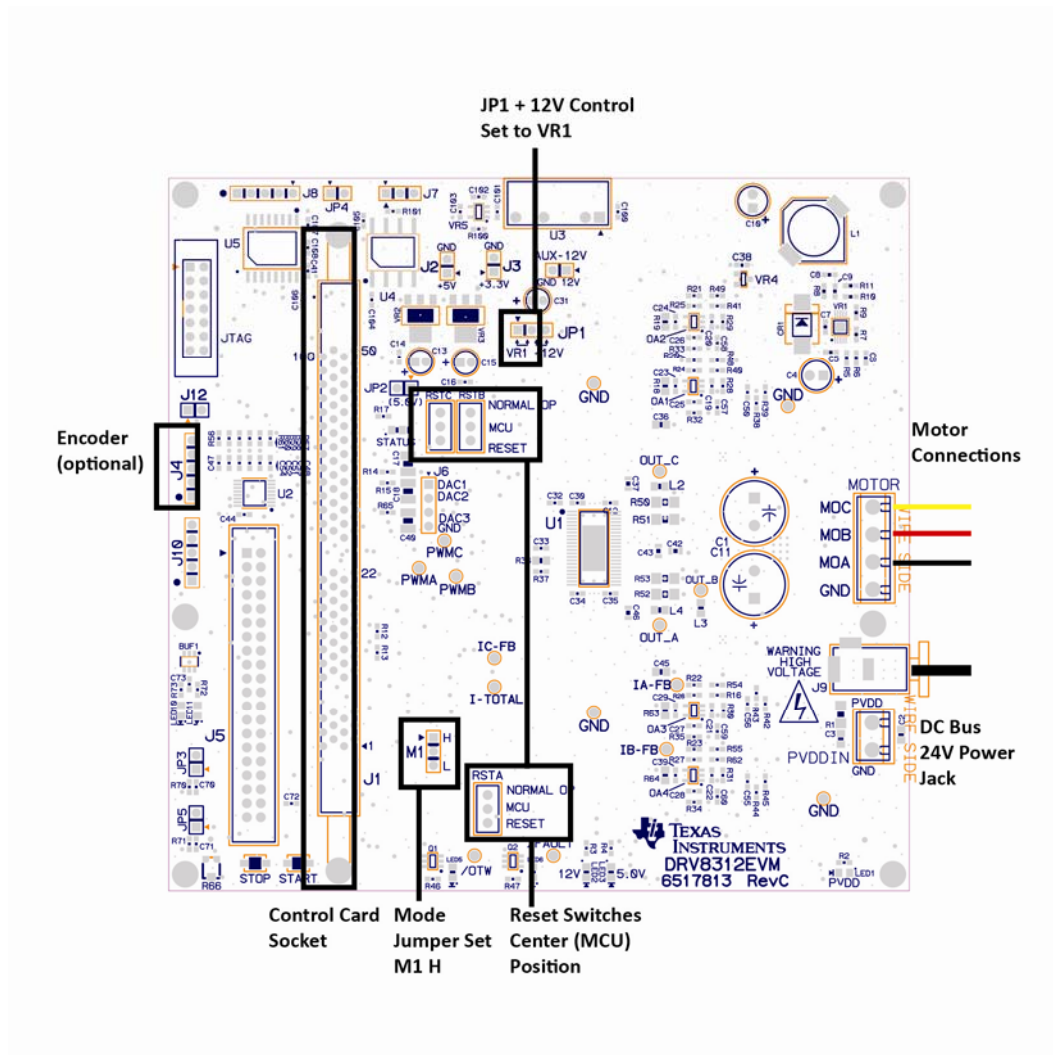
Figure 13 EVM Connections
