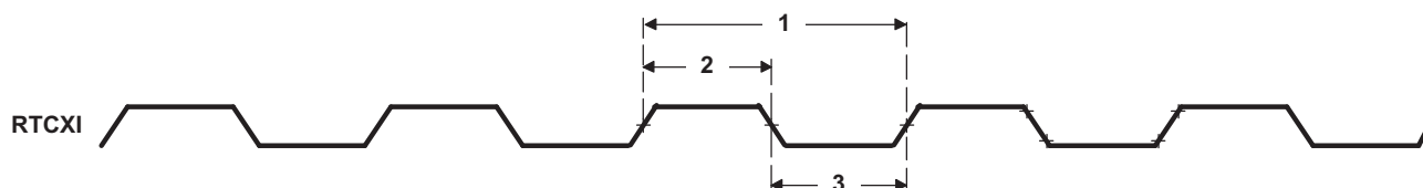
Figure 6-10. RTCXI Timing
