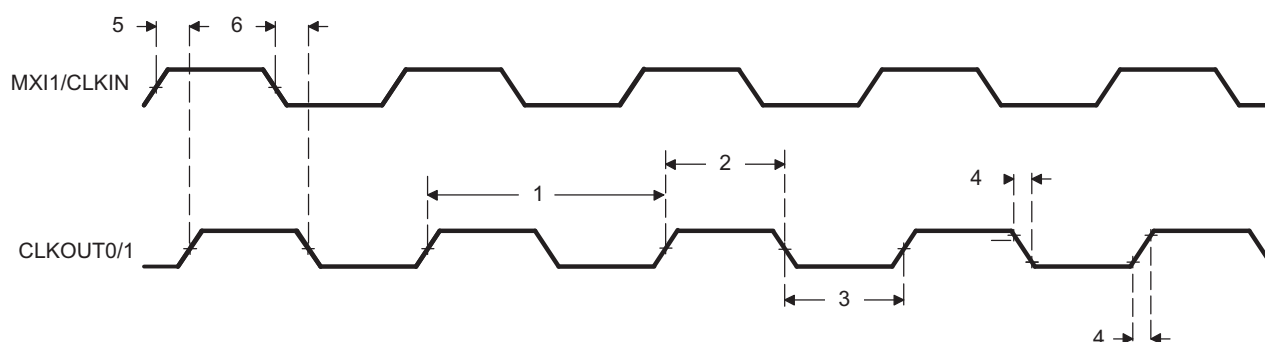
Figure 6-7. CLKOUT1 Timing
