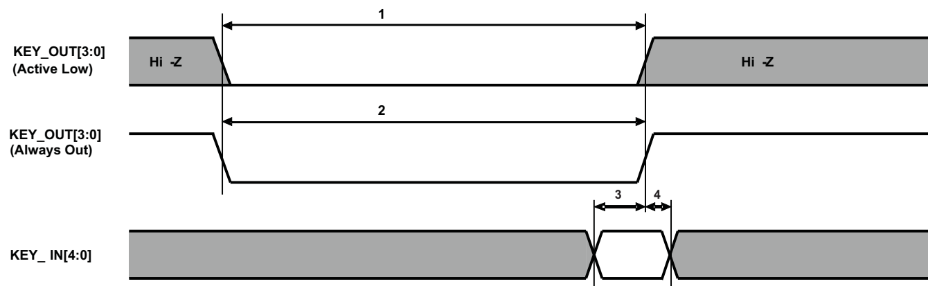
Figure 6-67. Key Scan Timing
