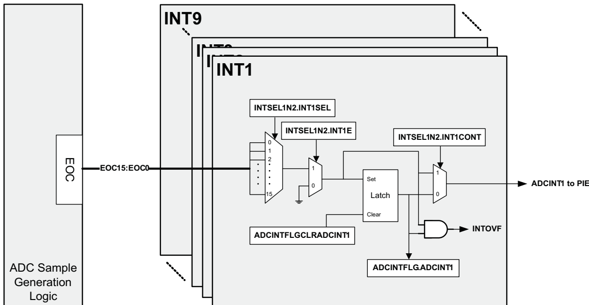
Figure 7. Interrupt Structure
