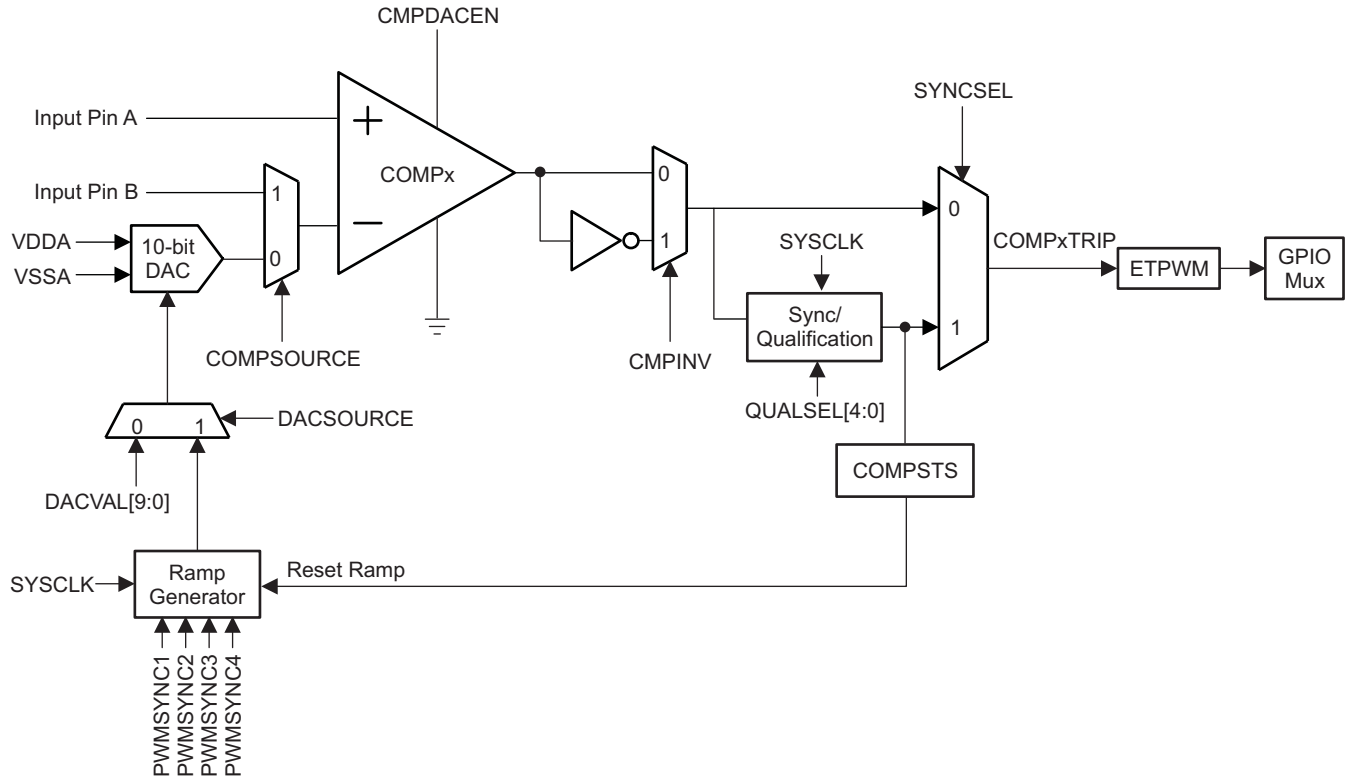
Figure 39. Comparator Block Diagram
