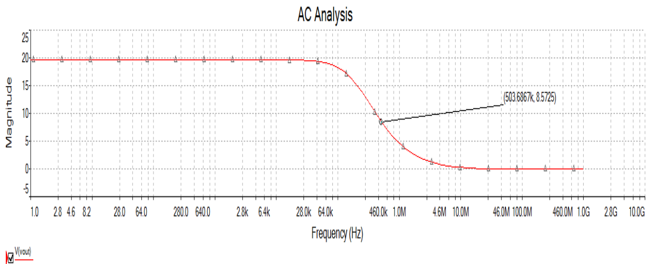
Fig 1: OPA604 output voltage with Rload=1kohm.
