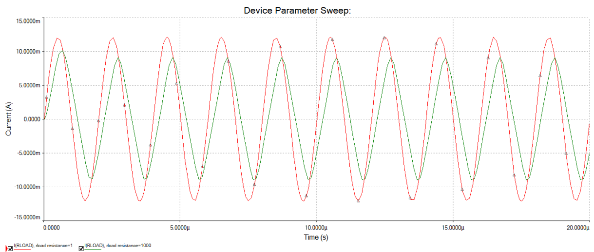
Figure 1: Current output at 500kHz (Rload=1ohm, 1kohm)
