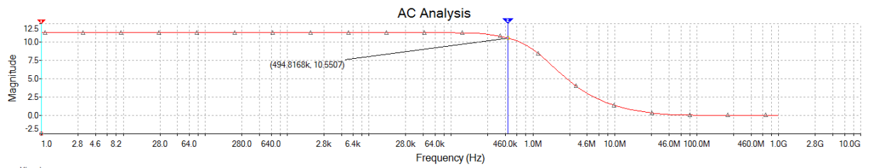
Figure 3: Ac analysis a) Magnitude (dB), b) Phase
