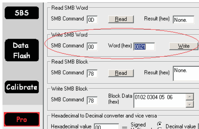
Figure A-4. Writing One-Word MAC Command in the Pro Screen
