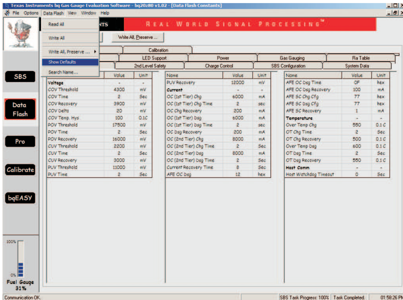
Figure 10. Data Flash Screen in bqEVS Showing Default Parameters
