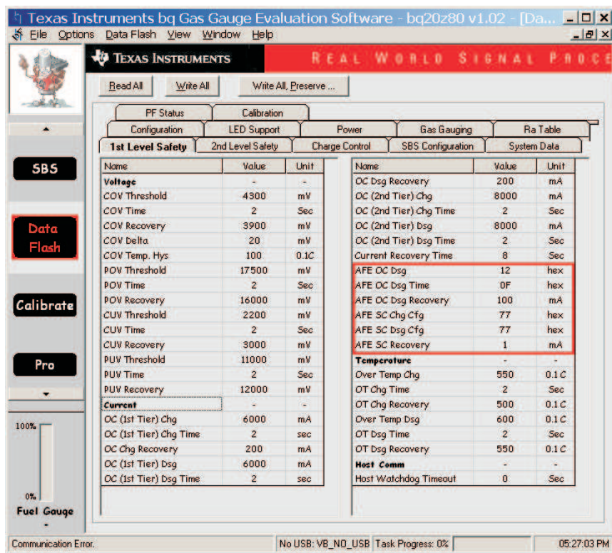
Figure A-7. Modifying AFE Registers
