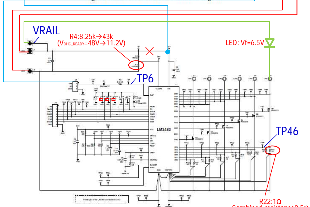
Figure 1. Circuit diagram of the LM3463 evaluation board
