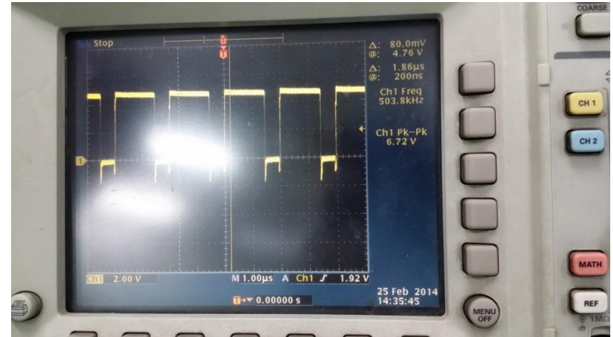
Nomal PH1(11Pin)PH2(12Pin),CNW3V3_PH
