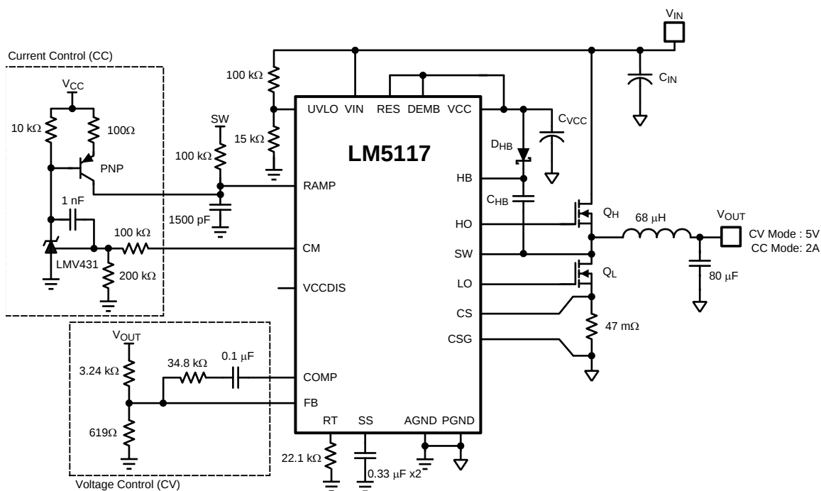
Figure 23. Constant Voltage Regulator with Accurate Current Limit
