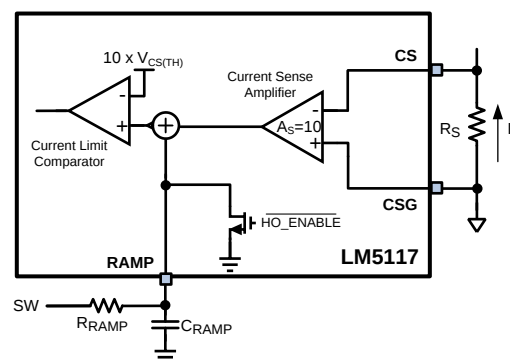
Figure 10. RAMP Generator and Current Limit Circuit
