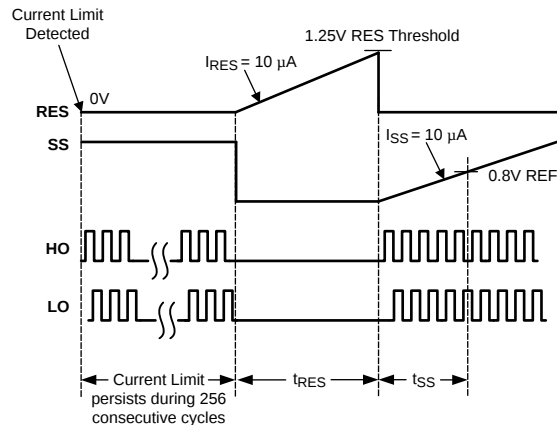
Figure 13. Hiccup Mode Current Limit Timing Diagram
