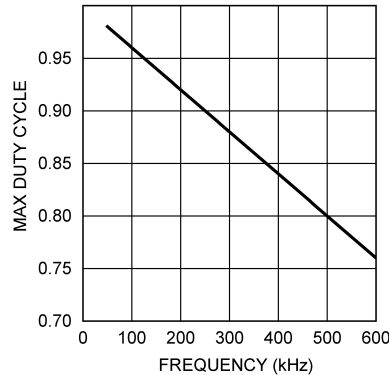
Figure 17. Maximum Duty Cycle vs Switching Frequency
