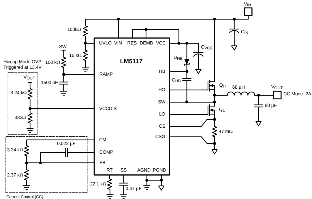
Figure 22. Constant Current Regulator with Hiccup Mode Output OVP
