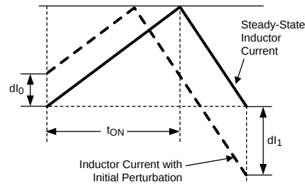
Figure 18. Effect of Initial Perturbation when dl_1/dl_0 < -1
