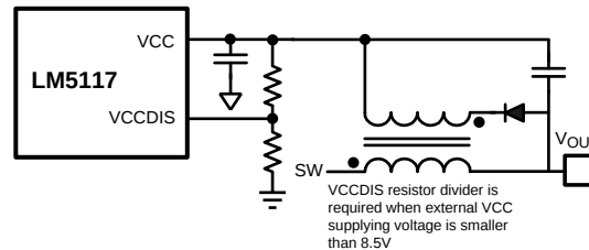
Figure 6. External VCC Supply for V_{OUT} < 6V
