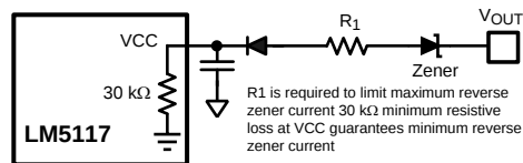
Figure 7. External VCC Supply for 14.5V < V_{OUT}
