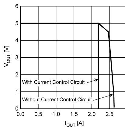
Figure 24. Current Limit Comparison
