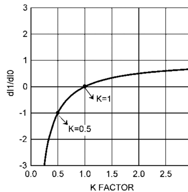
Figure 19. dl_1/dl_0 vs K Factor
