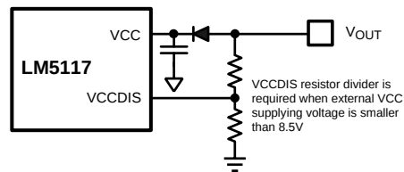
Figure 5. External VCC Supply for 6V < V_{OUT} < 14.5V
