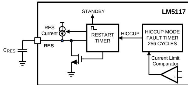
Figure 14. Hiccup Mode Current Limit Circuit
