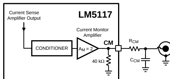
Figure 16. Current Monitor
