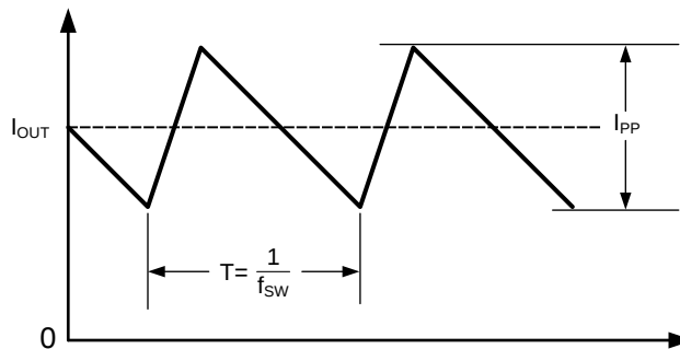
Figure 12. Inductor Current
