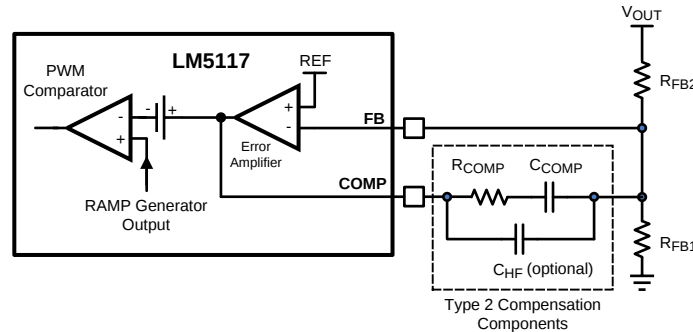
Figure 11. Feedback Configuration and PWM Comparator
