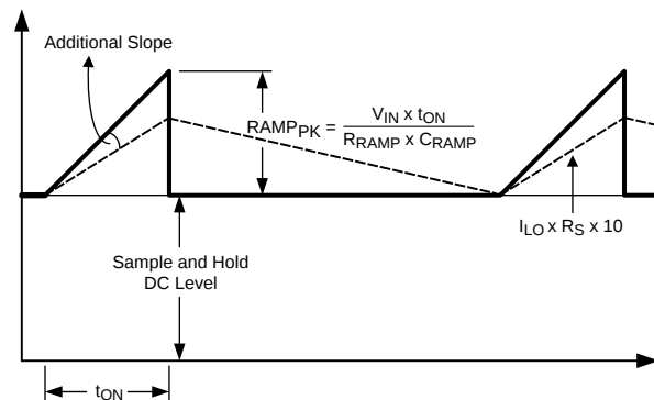
Figure 9. Composition of Emulated Current Sense Signal
