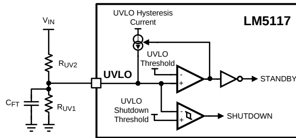
Figure 8. UVLO Configuration
