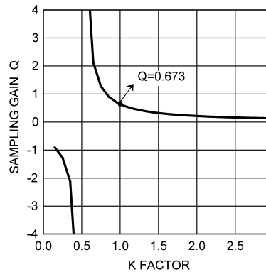
Figure 20. Sampling gain Q vs K Factor
