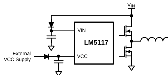
Figure 4. VIN Configuration for V_{VIN} < V_{VCC}
