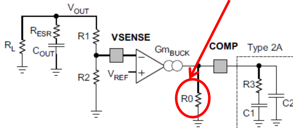
Figure 18. Buck Compensation Components
