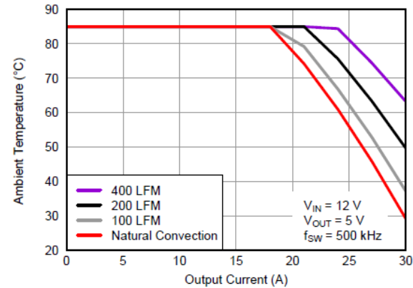
Figure 35. Safe Operating Area
