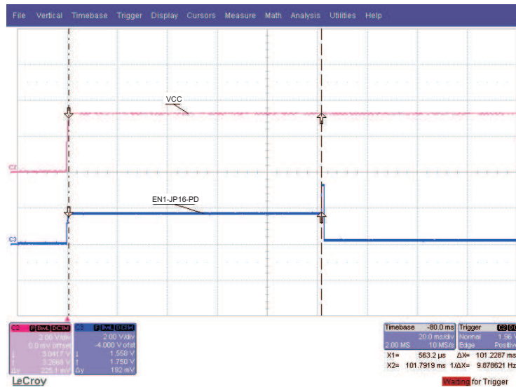
Figure 4. Power-Up Delay, With Parameter Change
