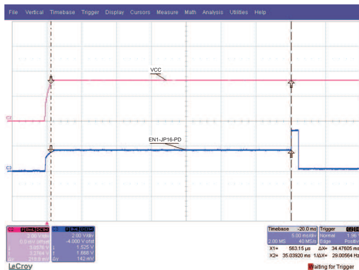
Figure 3. Power-Up Delay, no Parameter Change
