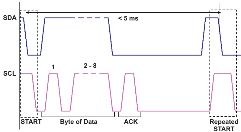
Figure 9. Byte Timeout Requirements
