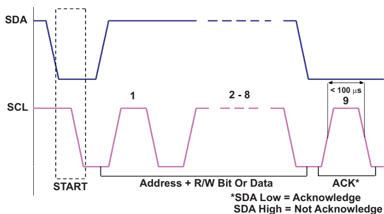
Figure 8. Acknowledge Bit Requirements
