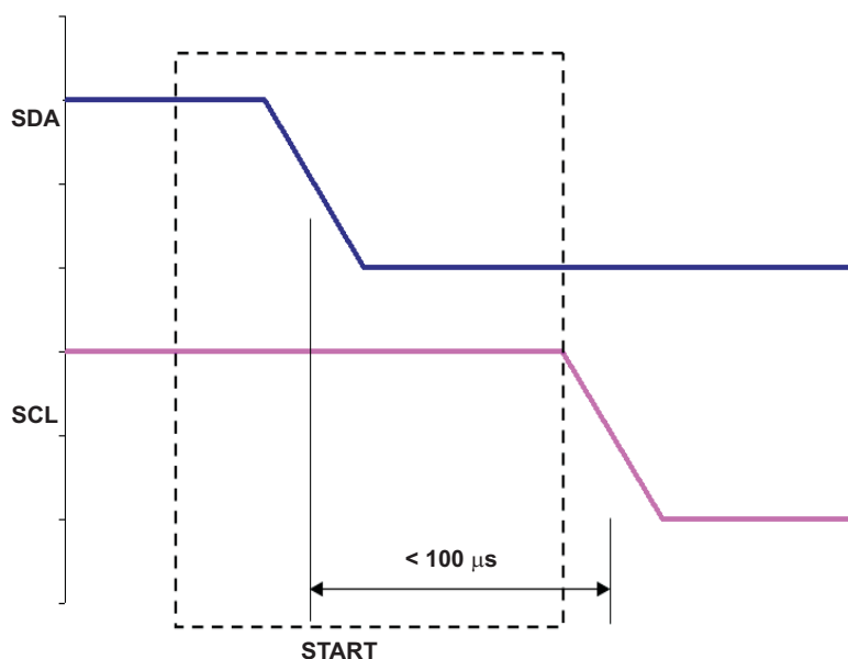
Figure 5. START Bit Requirement
