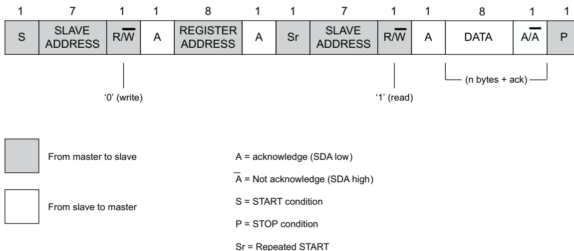
Figure 2. Read
