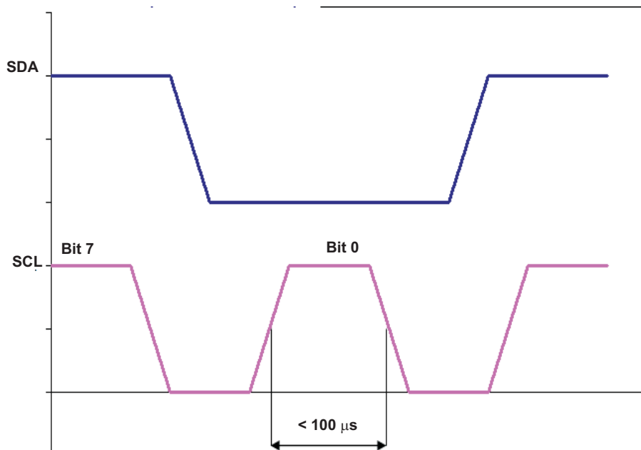
Figure 6. Eighth Bit of Write Command Requirements
