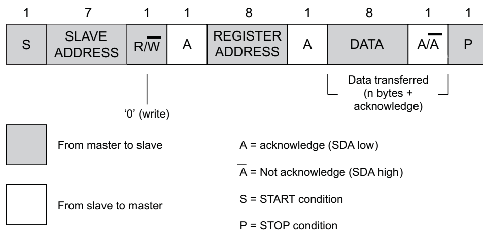
Figure 1. Write
