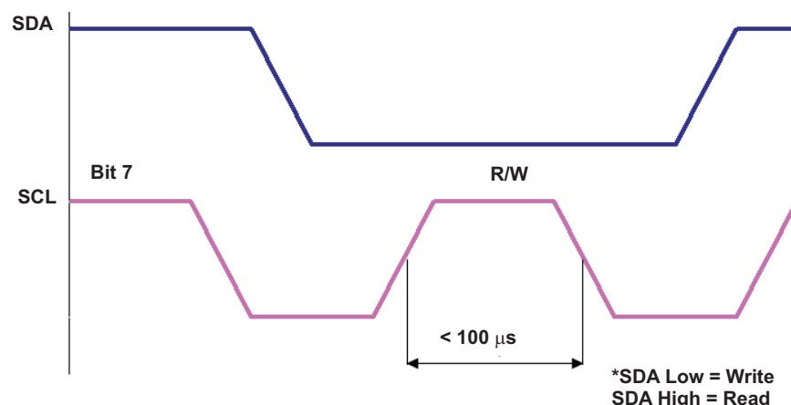
Figure 7. Read/Write Bit Requirements
