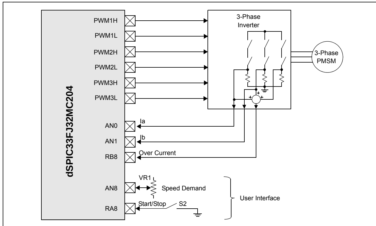
FIGURE 4: SYSTEM OVERVIEW
