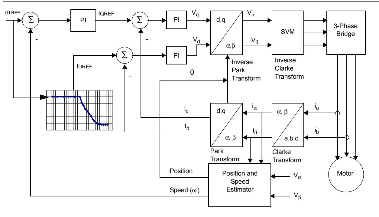
FIGURE 6: VECTOR CONTROL BLOCK DIAGRAM
