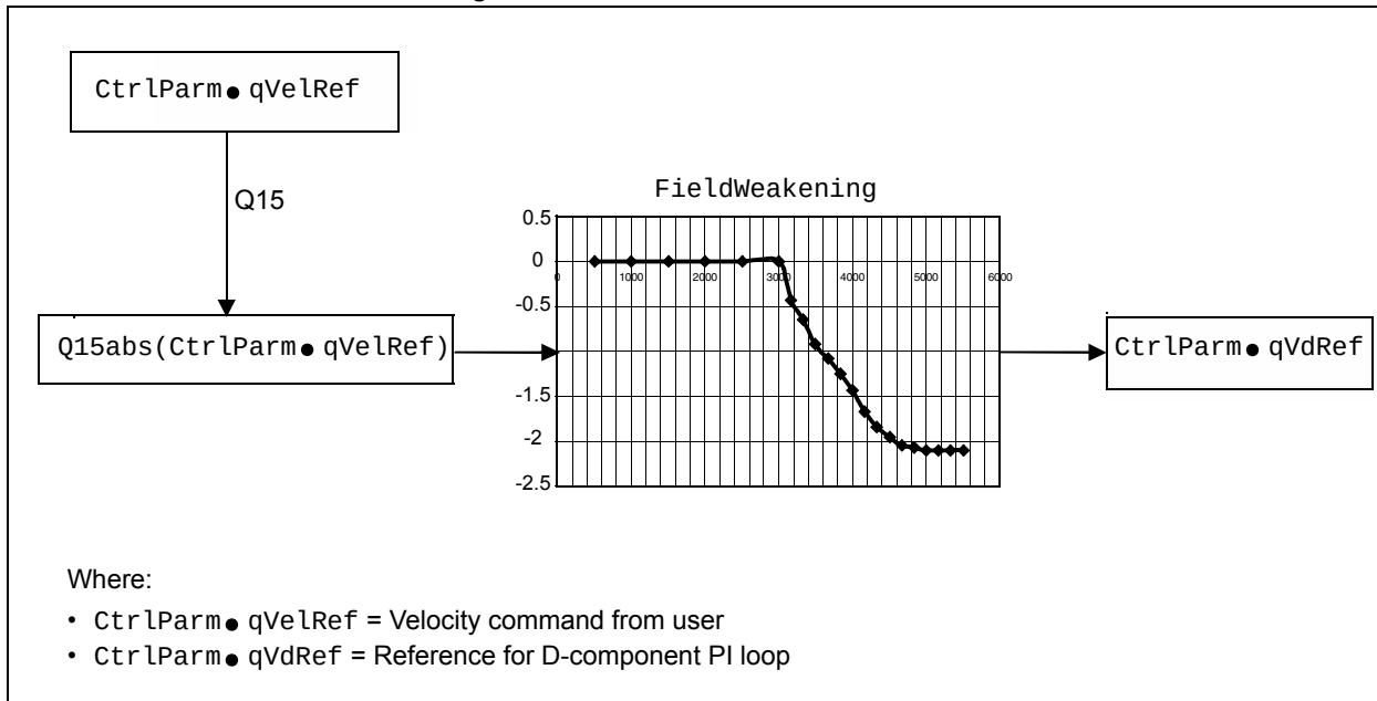
FIGURE 21: Fieldweakening FUNCTION BLOCK DIAGRAM
