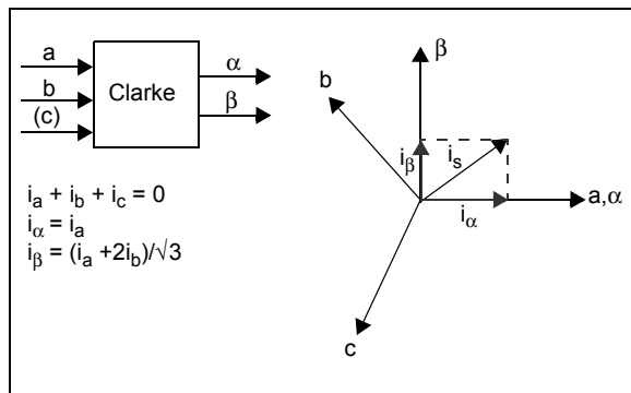
FIGURE 7: CLARKE TRANSFORM
