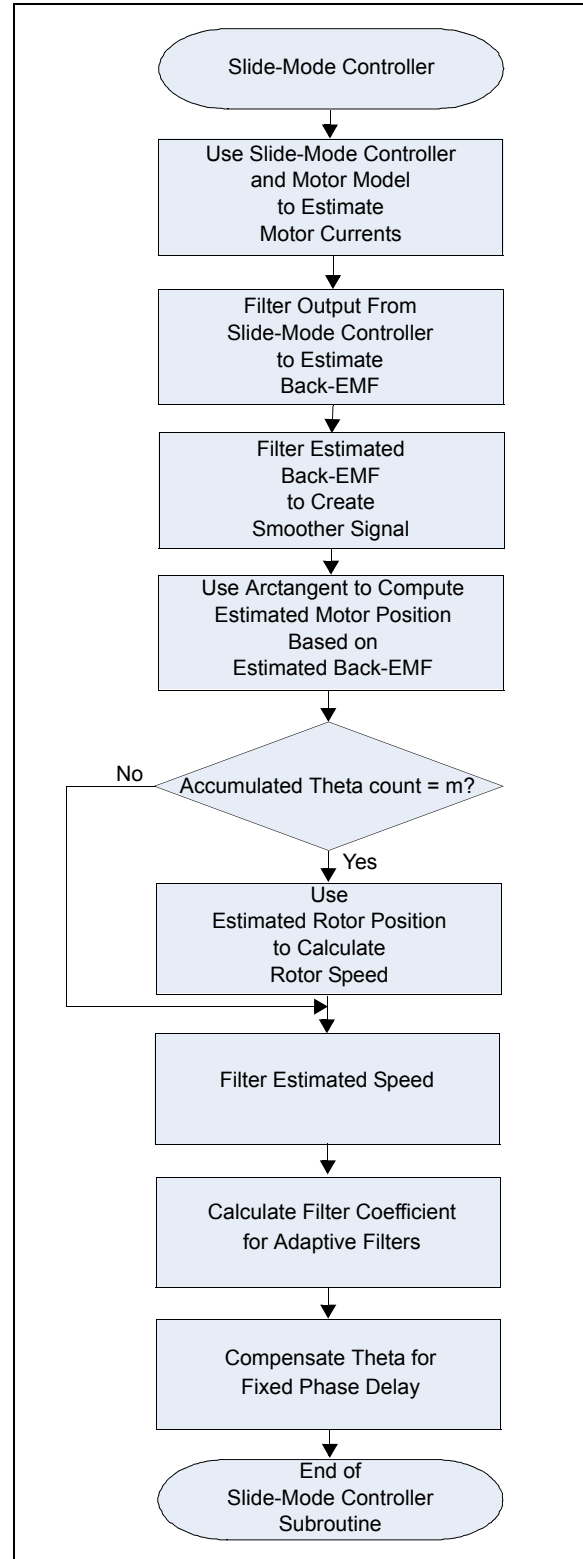
FIGURE 28: MOTOR POSITION AND SPEED ESTIMATION
