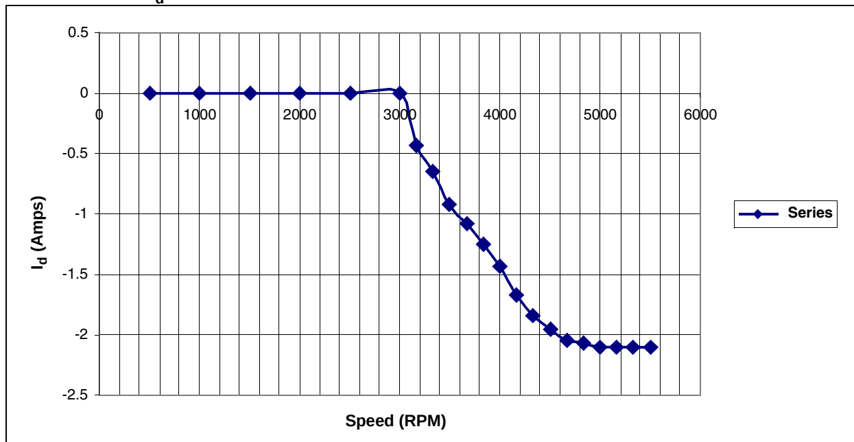
FIGURE 22: I_d vs. SHAFT RPM OF MOTOR
