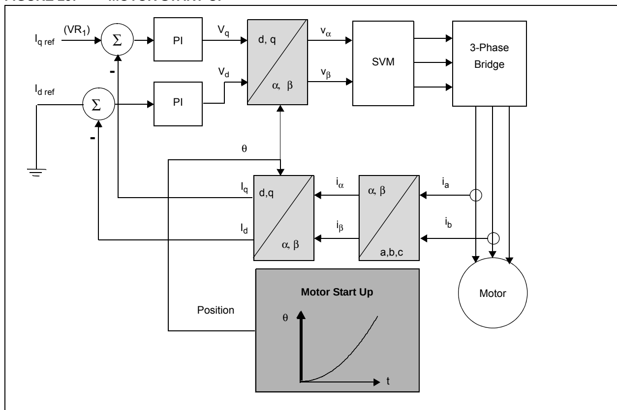
FIGURE 29: MOTOR START-UP
