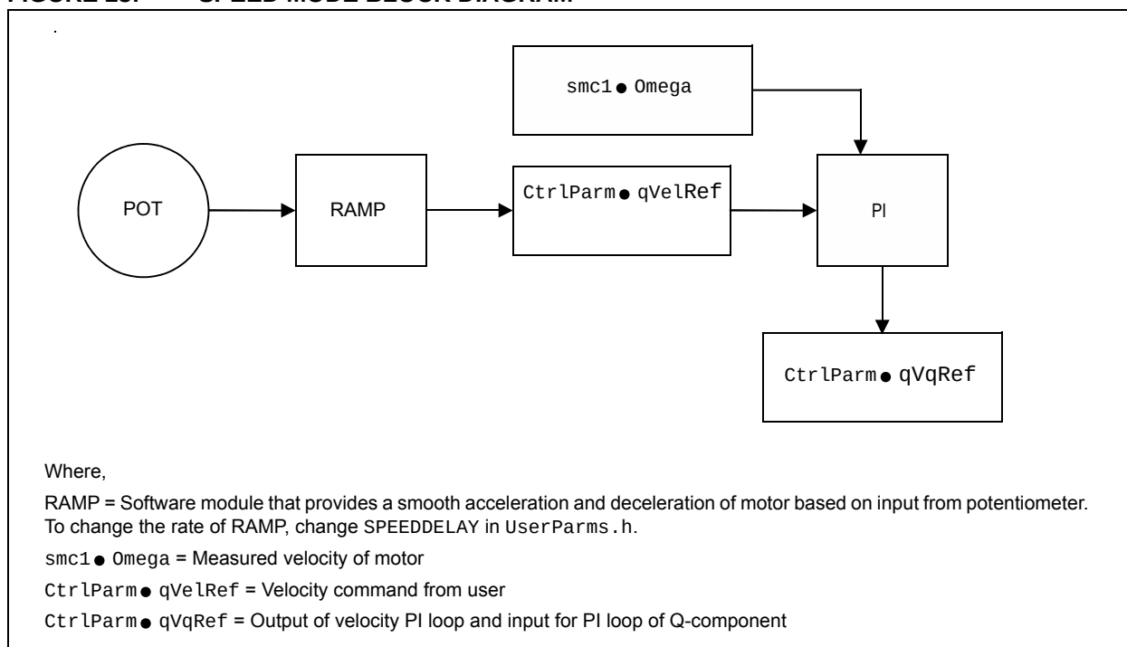
FIGURE 23: SPEED MODE BLOCK DIAGRAM
