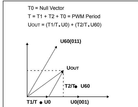
FIGURE 13: AVERAGE SVM
