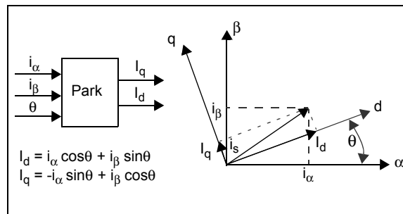
FIGURE 8: PARK TRANSFORM
