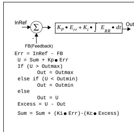
FIGURE 9: PI CONTROL
