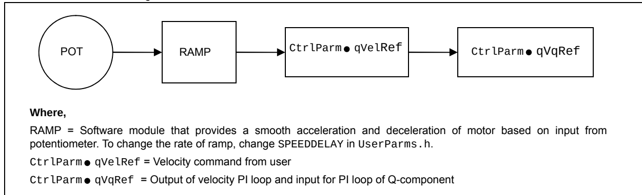
FIGURE 24: TORQUE MODE BLOCK DIAGRAM
