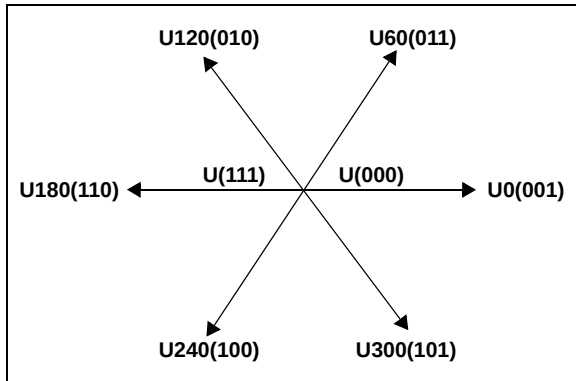
FIGURE 12: SVM
