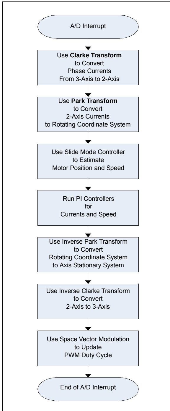
FIGURE 27: A/D INTERRUPT SUBROUTINE
