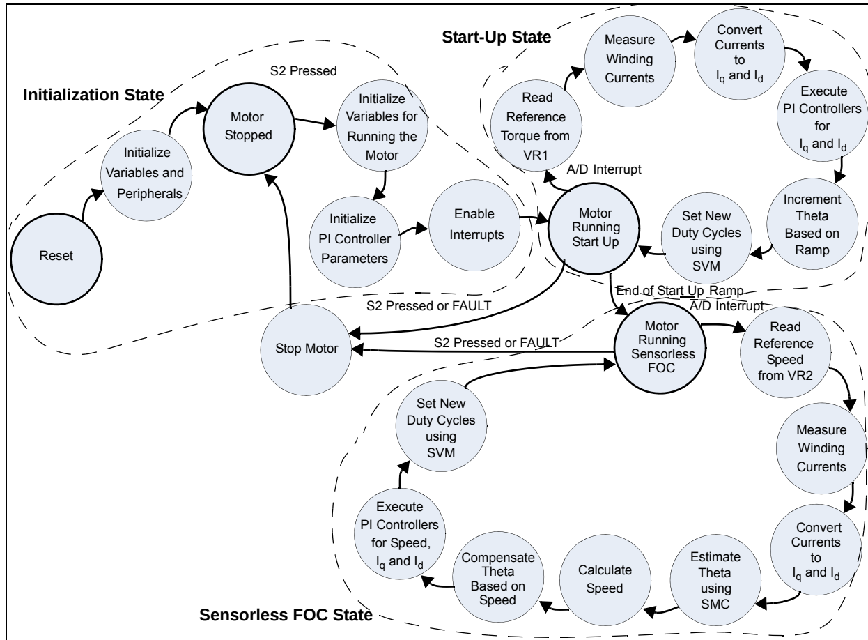
FIGURE 30: MAIN SOFTWARE STATE MACHINE
