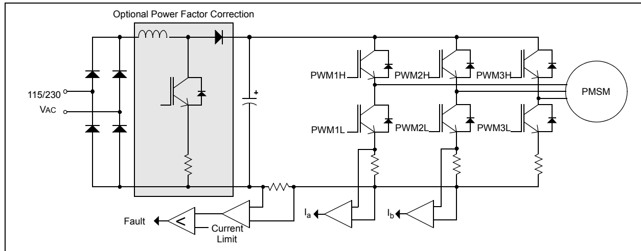
FIGURE 5: 3-PHASE TOPOLOGY
