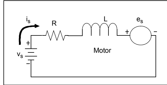
FIGURE 15: MOTOR MODEL
