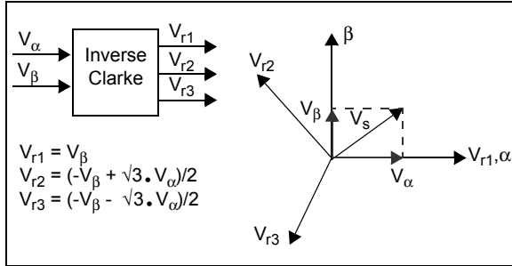
FIGURE 11: INVERSE CLARKE
