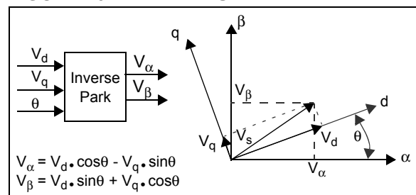
FIGURE 10: INVERSE PARK
