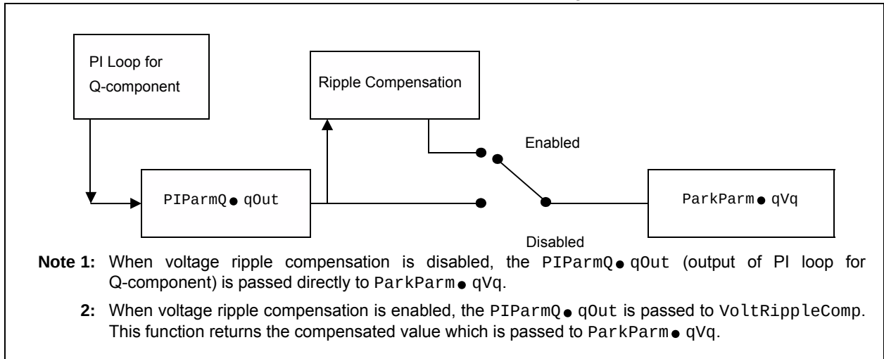
FIGURE 26: BUS VOLTAGE RIPPLE COMPENSATION FOR Q-AXIS CURRENT (1,2)
