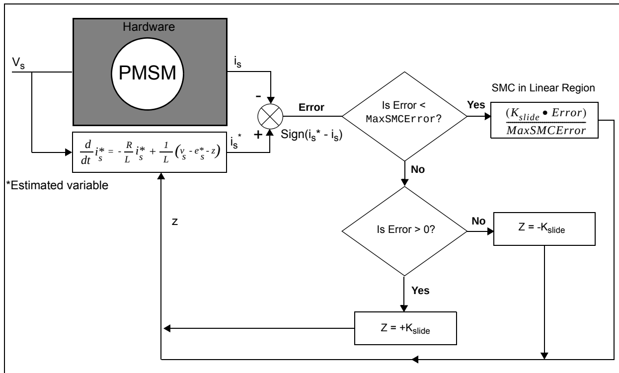
FIGURE 17: CURRENT OBSERVER BLOCK DIAGRAM
