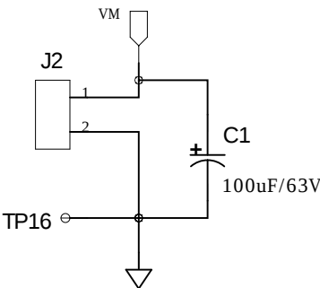
Input Connector
