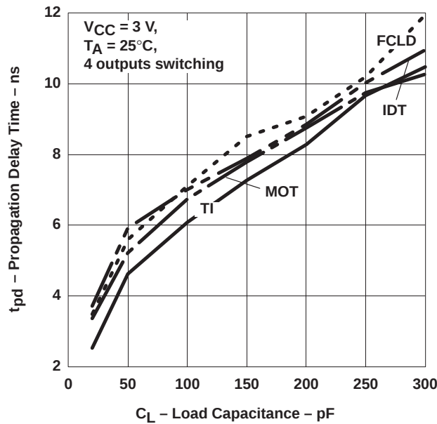
(c) '245 - t_{PLH}
