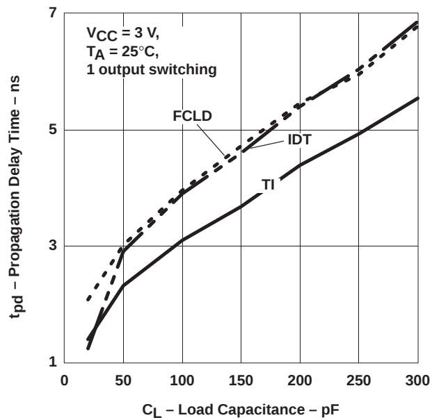
(b) '16245 - tPHL
