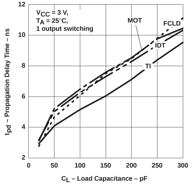
(b) '245 - t_{PHL}
