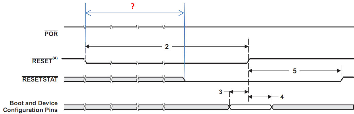
Figure 7-11. Warm Reset Timing
