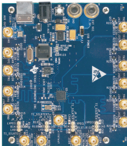
Figure 1. CDCE62005EVM Evaluation Board
