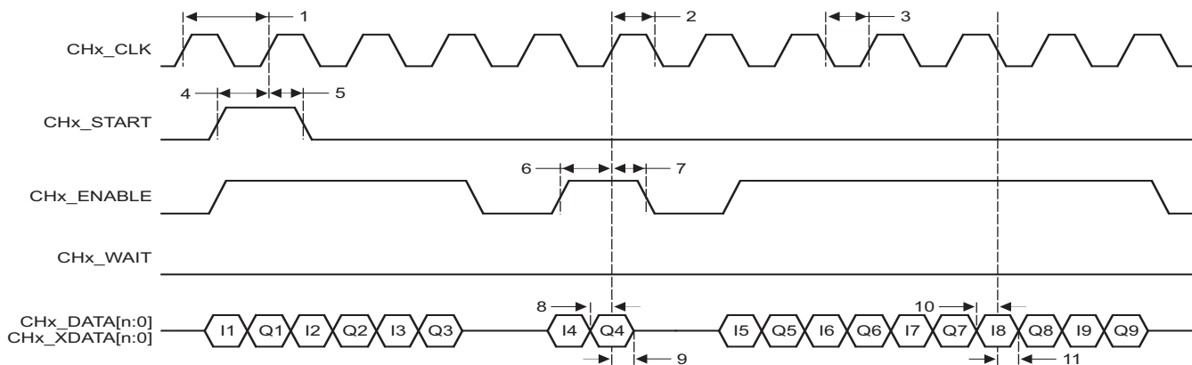
Figure 7-57 UPP Double Data Rate (DDR) Receive Timing
