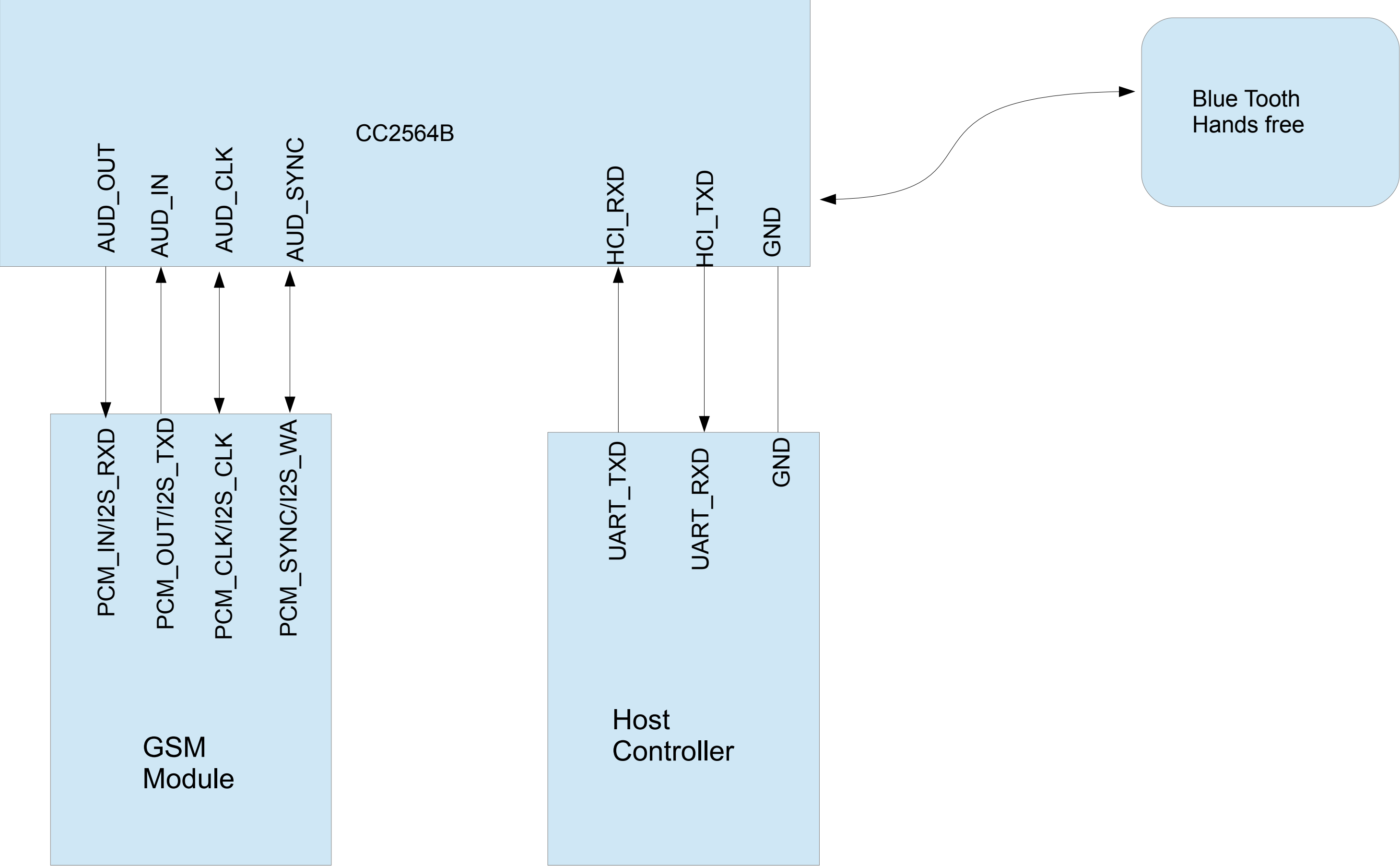
Blue tooth Digital Audio Interface
