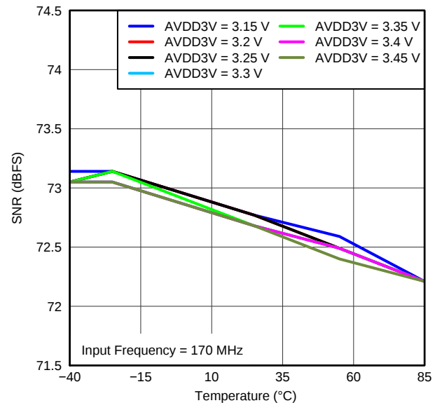
Figure 64. SNR vs AVDD_BUF SUPPLY AND TEMPERATURE (170 MHz)
