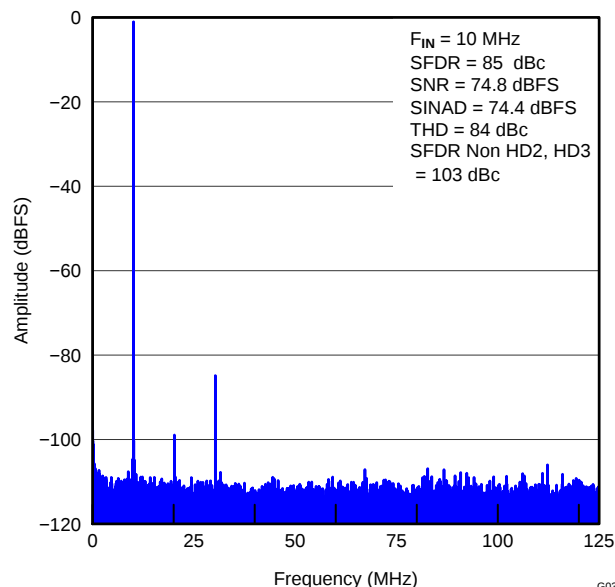
Figure 44. FFT FOR 10-MHz INPUT SIGNAL (2.5- V_{PP} Full-Scale)
