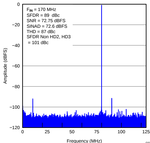
Figure 42. FFT FOR 170-MHz INPUT SIGNAL
