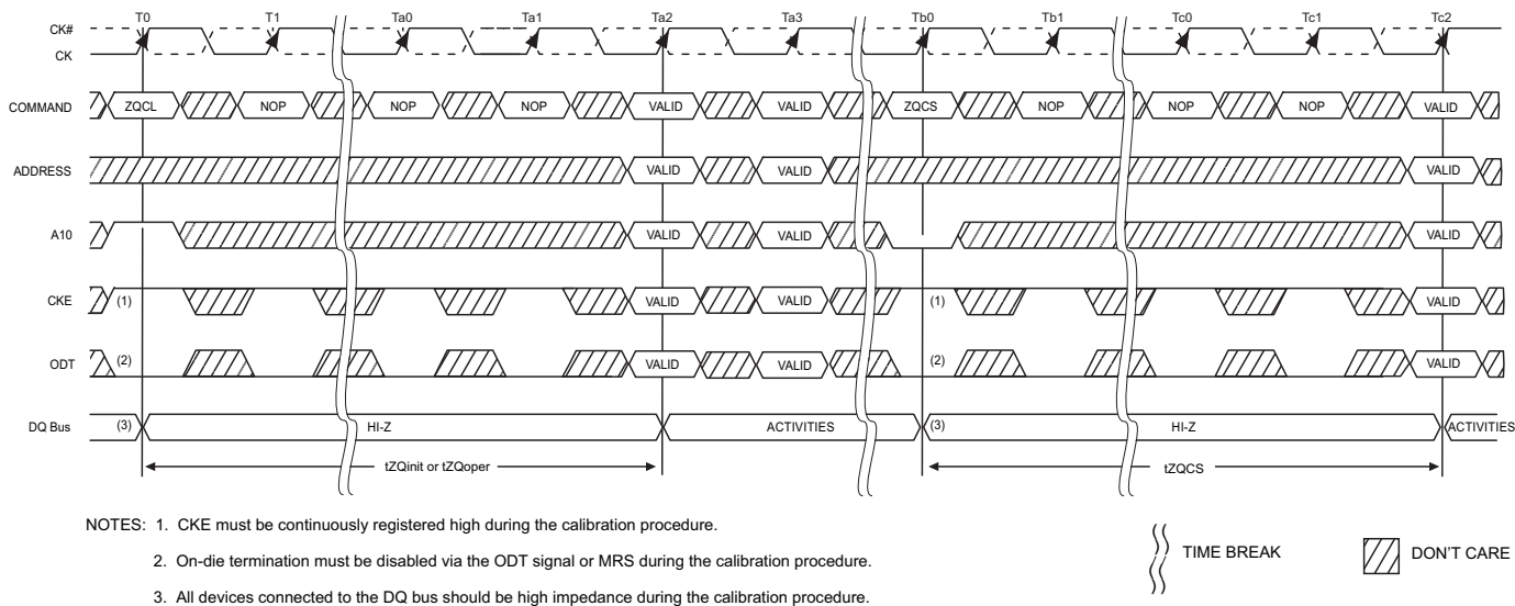
Figure 90 — ZQ Calibration Timing
