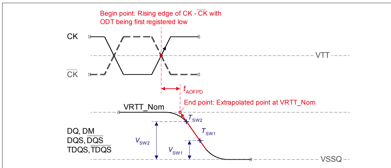
Figure 107 — Definition of t_{\text{AOFPD}}
