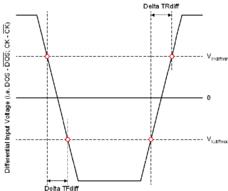
Figure 95 — Differential Input Slew Rate Definition for DQS, DQS# and CK, CK#
