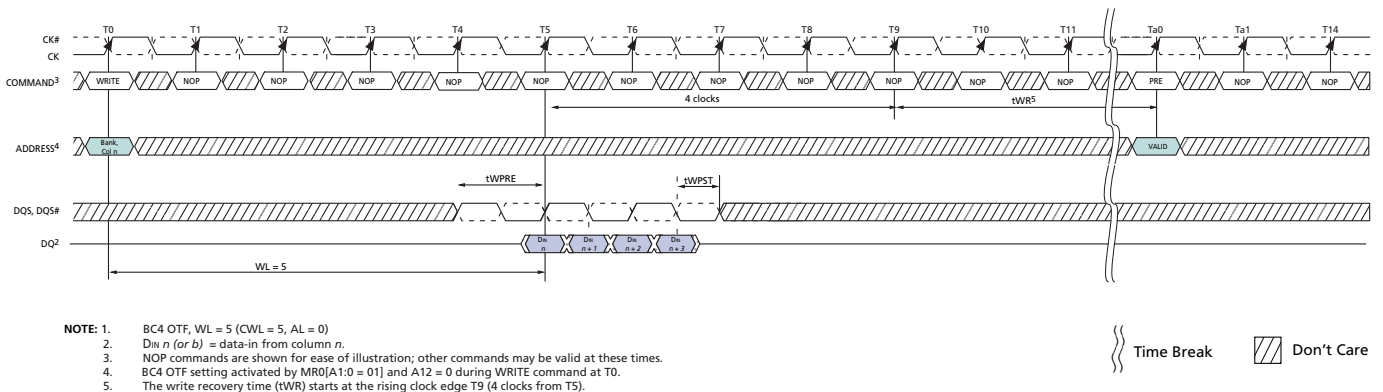
Figure 51 — WRITE (BC4) OTF to PRECHARGE Operation
