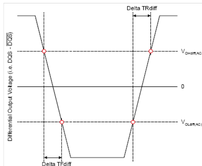
Figure 97 — Differential Output Slew Rate Definition
