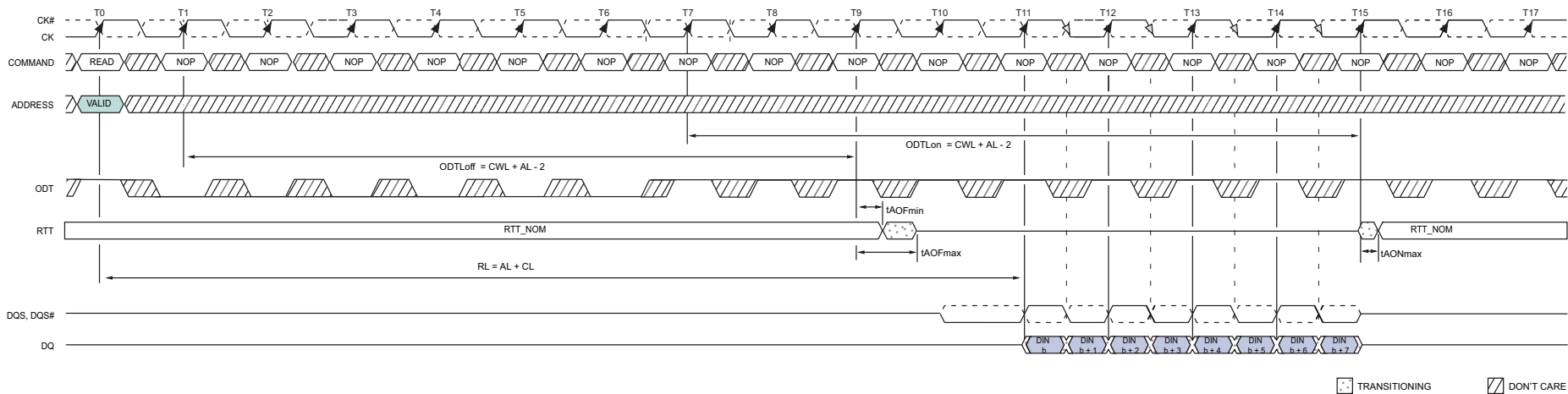
Figure 79 — ODT must be disabled externally during Reads by driving ODT low. (example: CL = 6 ; AL = CL - 1 = 5 ; RL = AL + CL = 11 ; CWL = 5 ; ODTLon = CWL + AL - 2 = 8 ; ODTLoff = CWL + AL - 2 = 8 )
