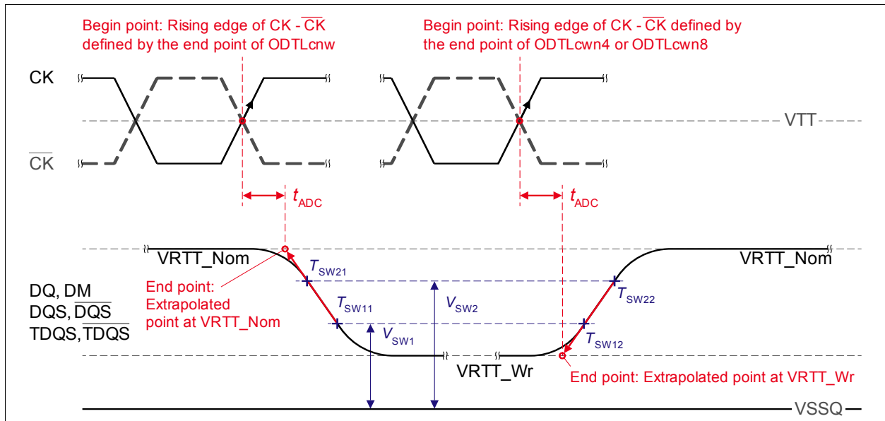
Figure 108 — Definition of t_{\text{ADC}}
