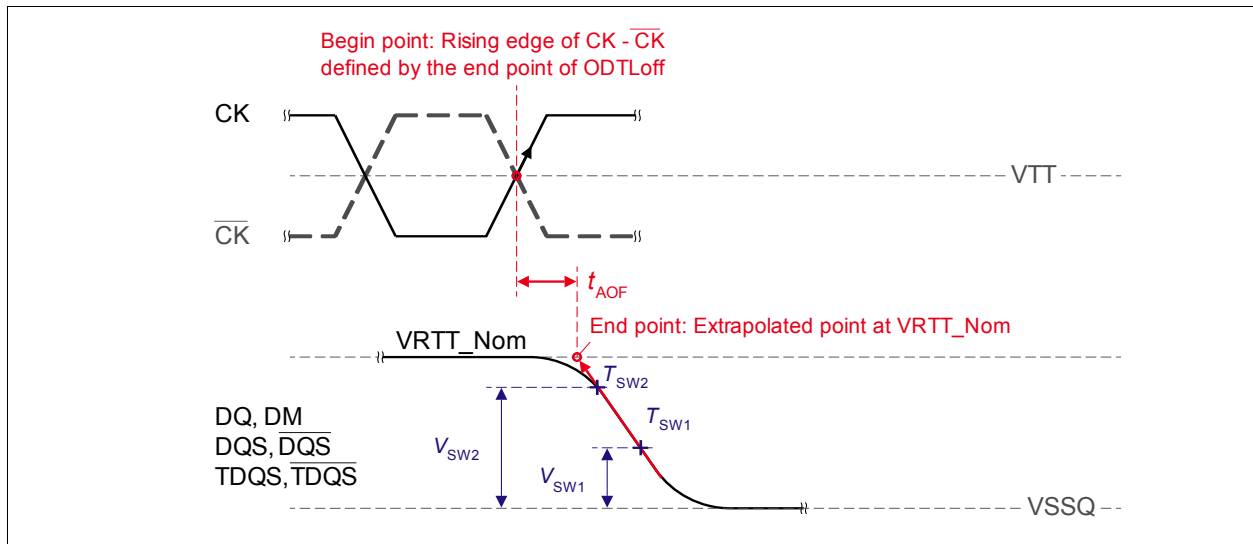
Figure 106 — Definition of t_{\text{AOF}}
