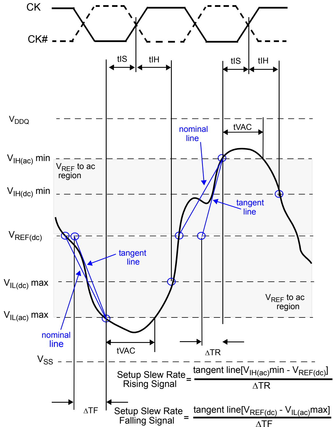
Figure 113 — Illustration of tangent line for setup time t_{IS} (for ADD/CMD with respect to clock)
