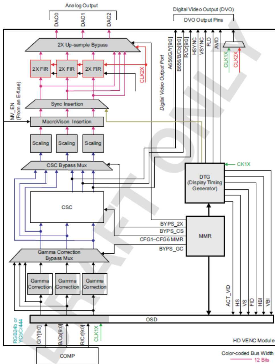
Figure 109. HD VENC Block Diagram
