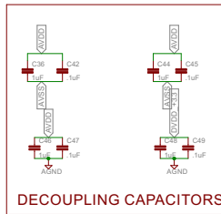
DECOUPLING CAPACITORS
