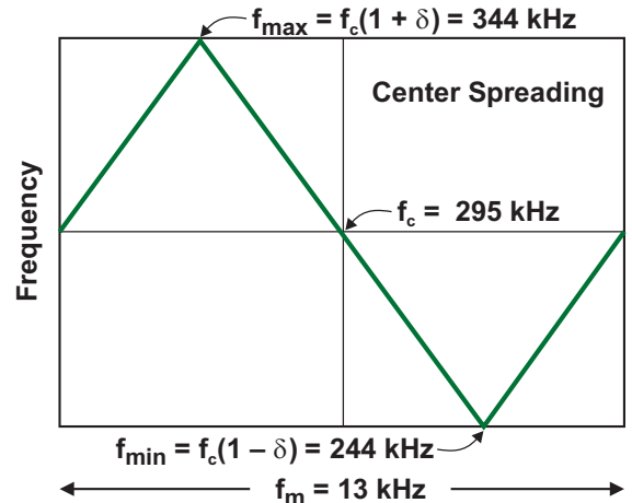
Fig. 11. Modulation waveform.
