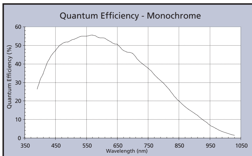
Figure 24: Quantum Efficiency—Monochrome
