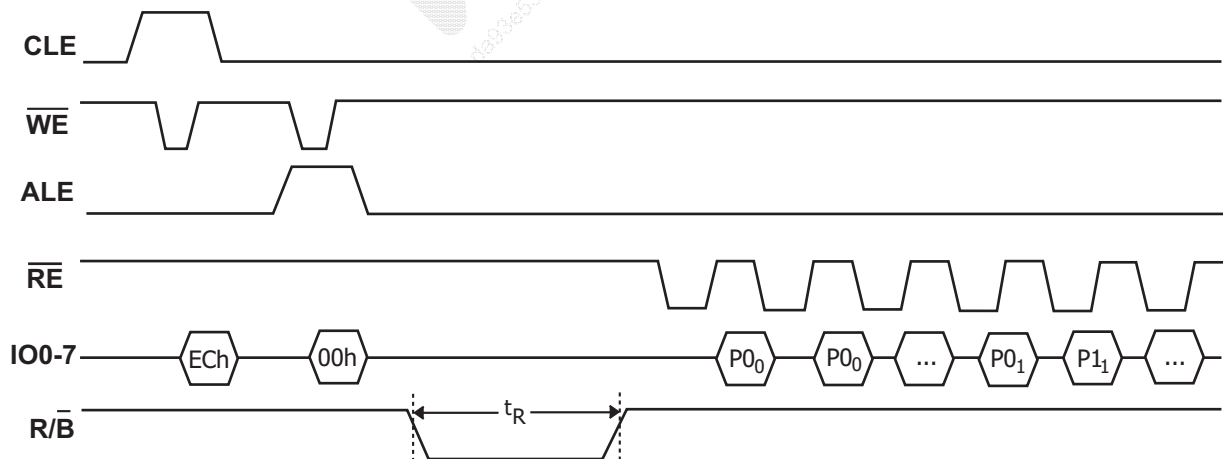
Figure 38: Read Parameter Page timings
