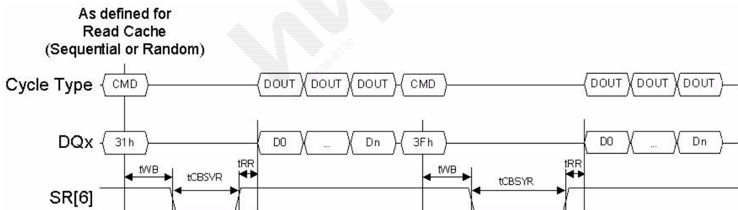
Figure 33: Read cache timings, end of cache operation
