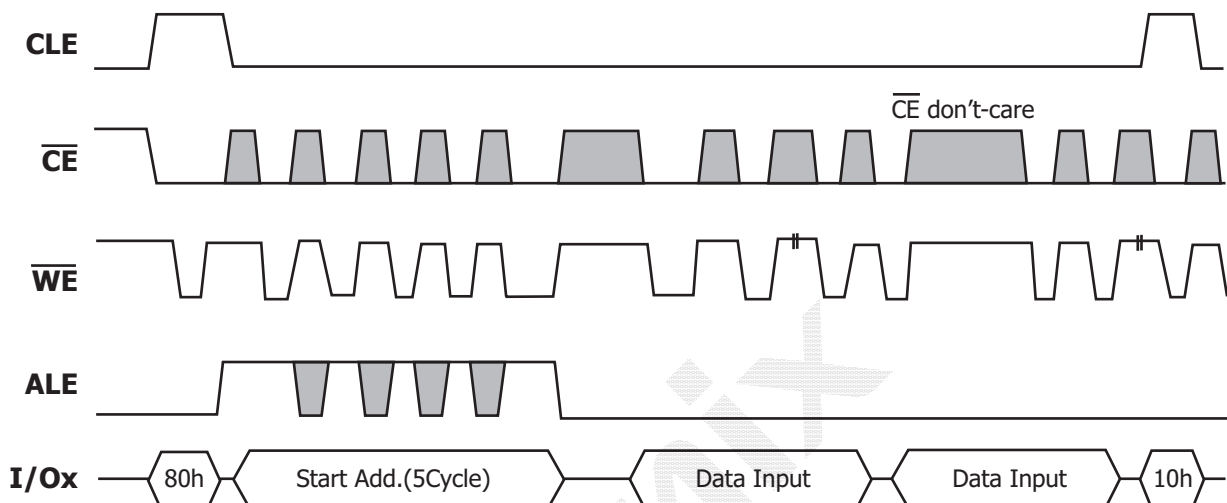
Figure 47: Program Operation with CE# don't-care.
