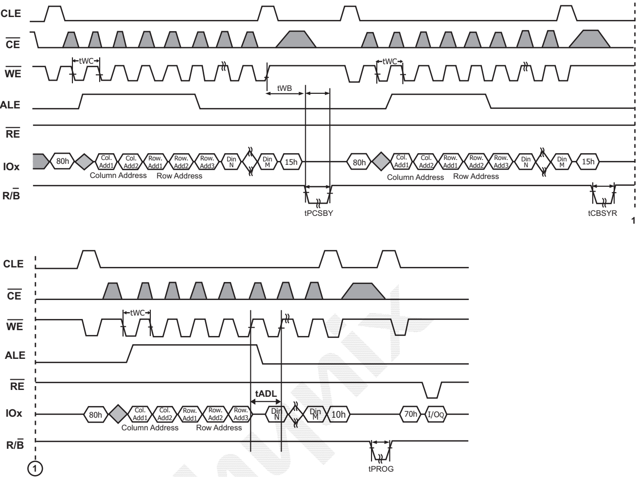
Figure 41: Cache program
