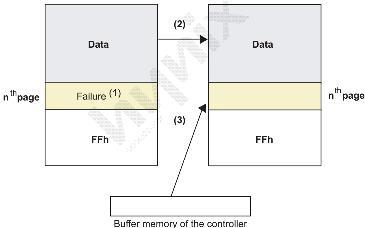
Figure 49 : Bad Block Replacement
