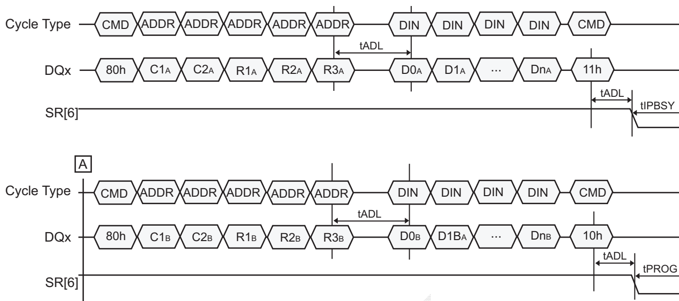
Figure 22 : Multiple plane page program (ONFI 1.0 protocol)
