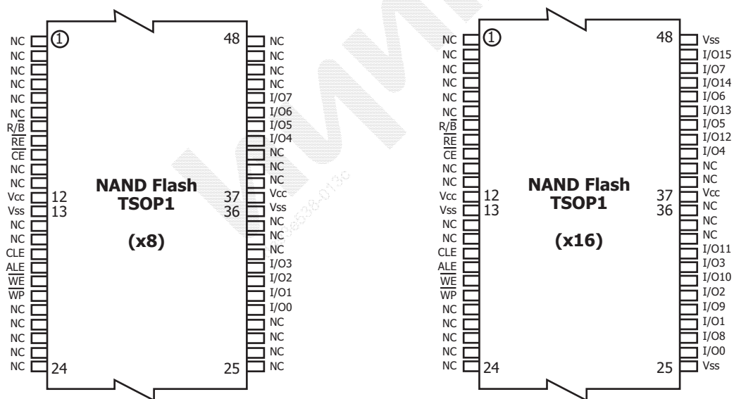
Figure 2. 48TSOP1 Contact, x8 and x16 Devic
