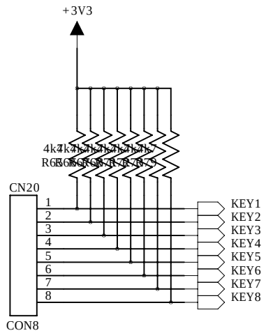
KEYPAD CONNECTOR
