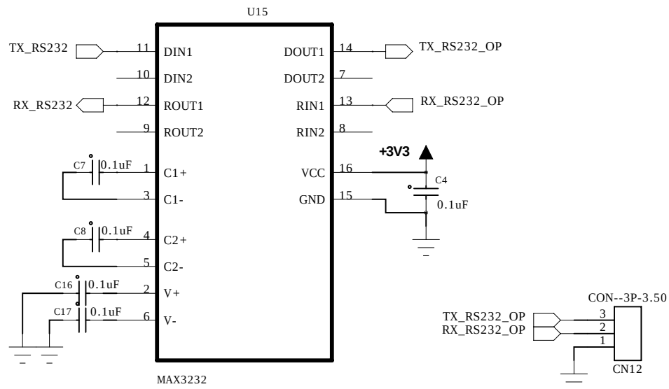
RS232
