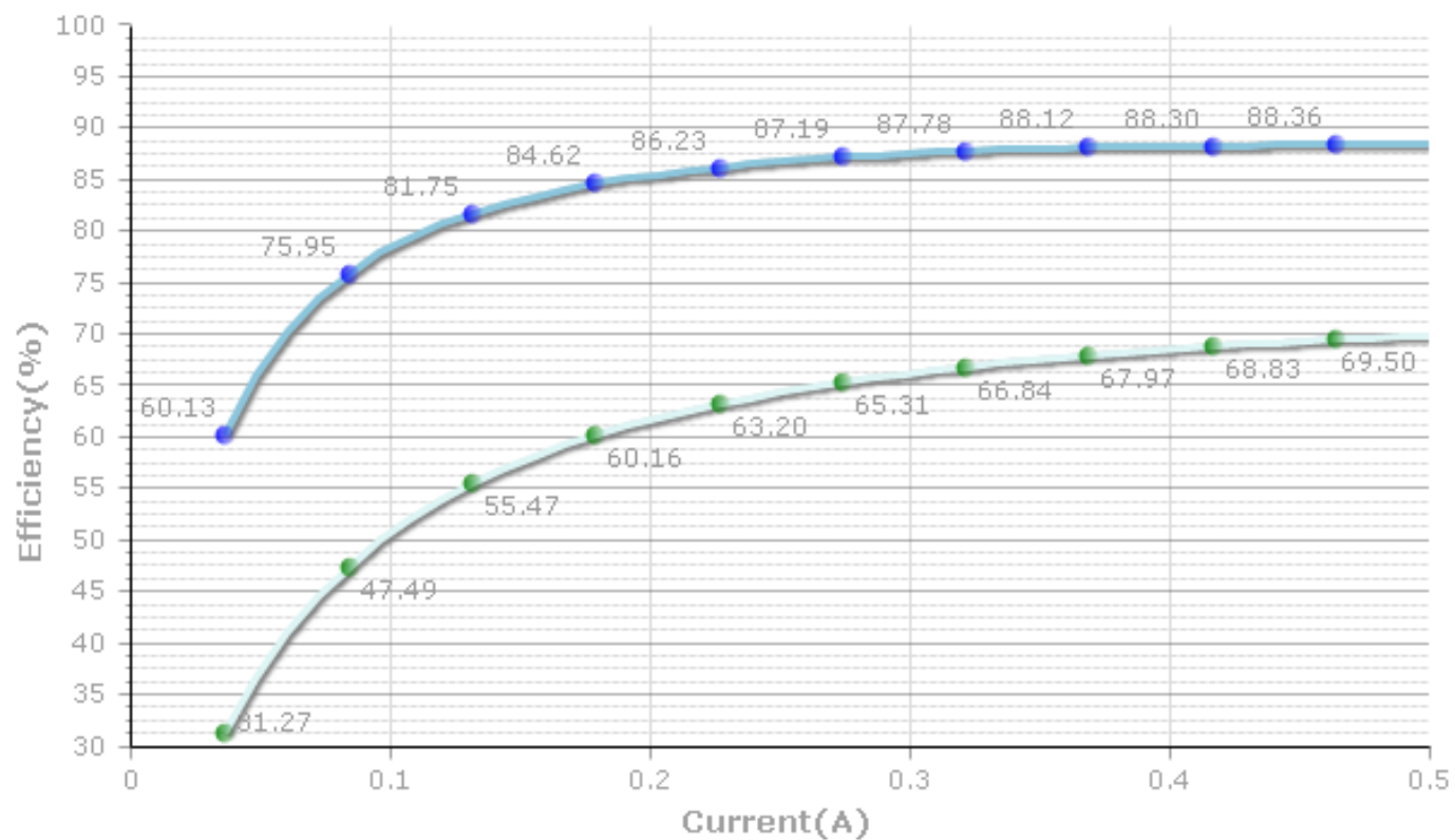
Efficiency - Output1
