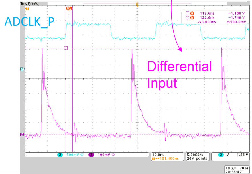
R:75ohm C:15pF Rs:10ohm
