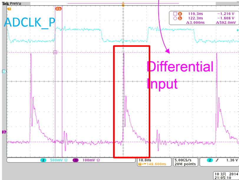
R:33ohm C:47pF Rs:10ohm
