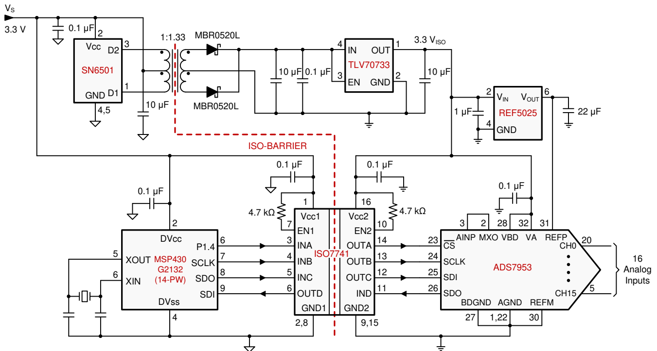
Figure 10-1. Isolated SPI for an Analog Input Module With 16 Input
