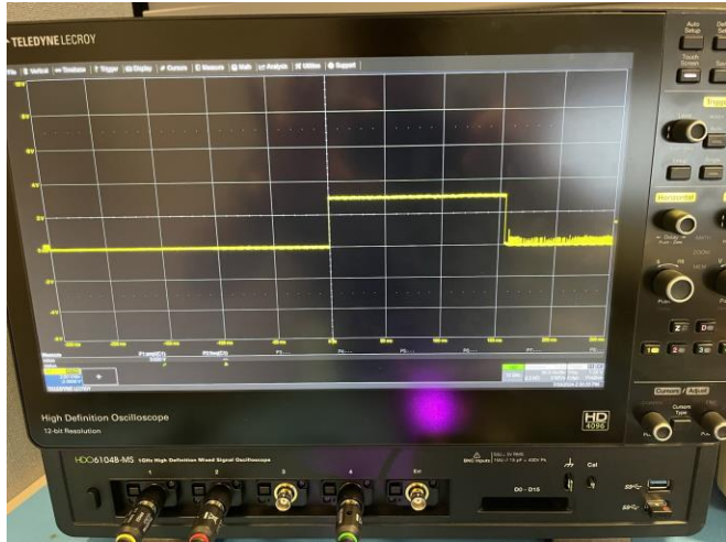
DD+ Pullup on power-cycle with No isolation
