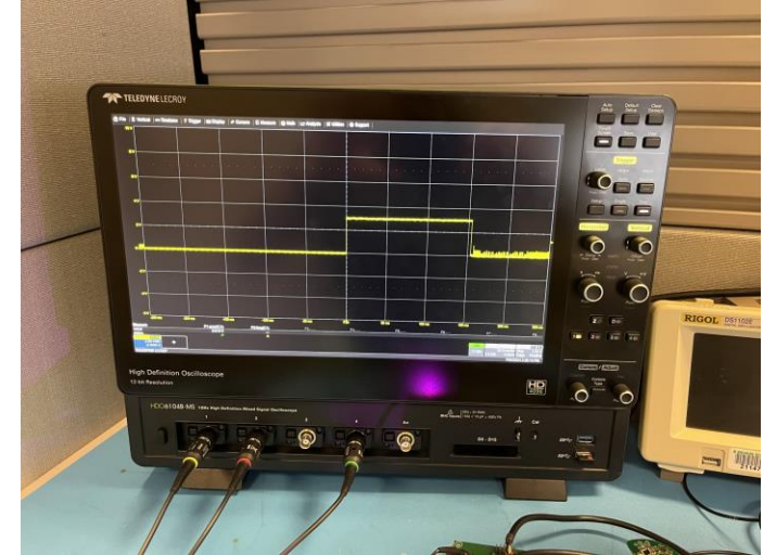
DD+ Pullup on power-cycle with Analog Device's ADUM4166
