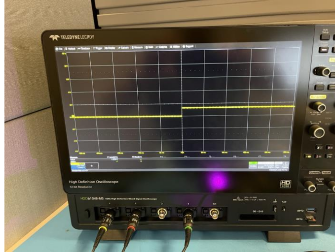
DD+ Pullup on power-cycle with TI's ISOUSB 211
