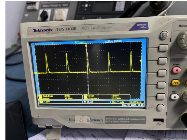
CAN high and low signal
