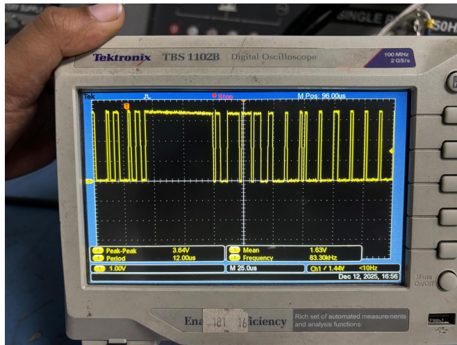
MCU CAN tx signal
