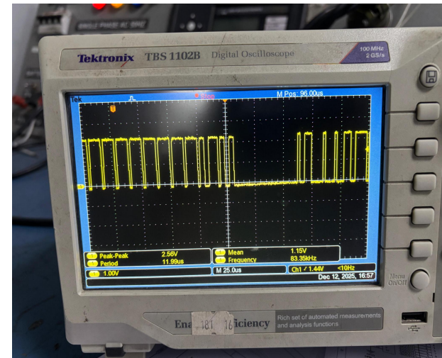
CAN high and low signal
