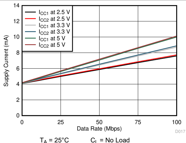
Figure 6-12. ISO7763 Supply Current vs Data Rate (With No Load)
