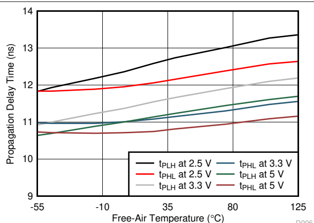
Figure 6-16. Propagation Delay Time vs Free-Air Temperature
