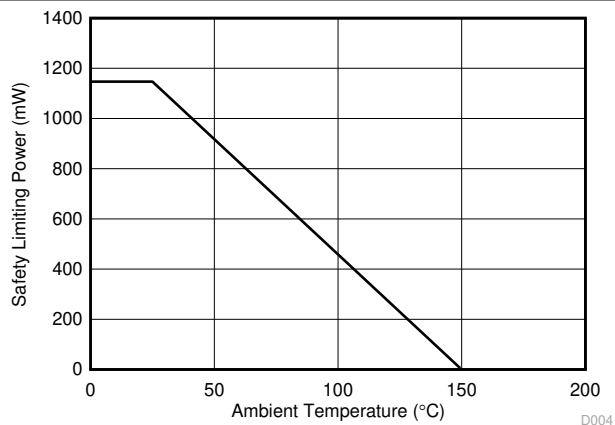
Figure 7-4. Thermal Derating Curve for Safety Limiting Power per VDE for DBQ-16 Package
