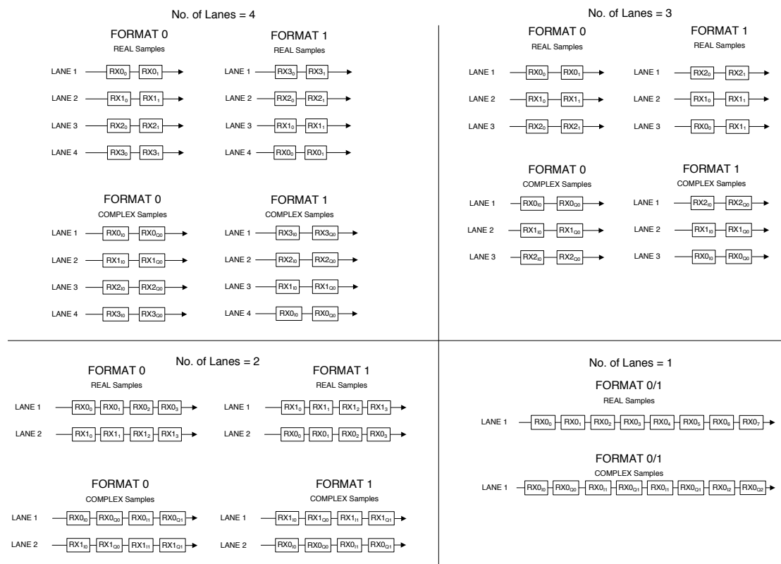
Figure 5.4: Lane formats and the order of receiving the data from the lanes
