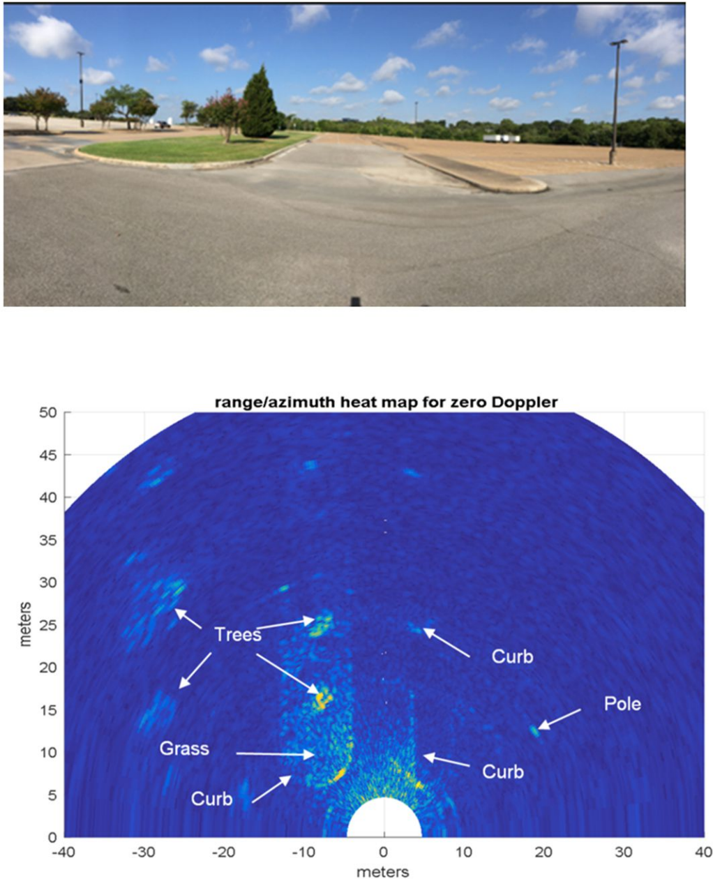
图 28. Parking Lot Curb Scene (Top), and Resulting Azimuth Range Heatmap (Bottom)
