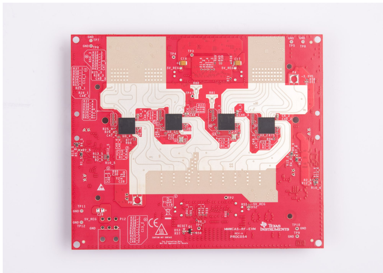
图 1. AWR2243 Four-Device Cascade Radar RF Radar Board
