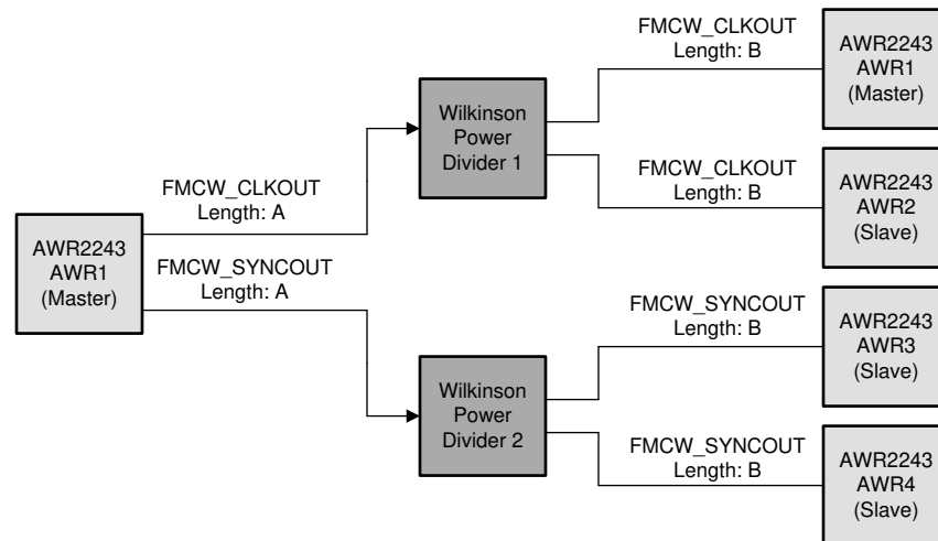
图 3. 20 GHz LO Distribution Block Diagram
