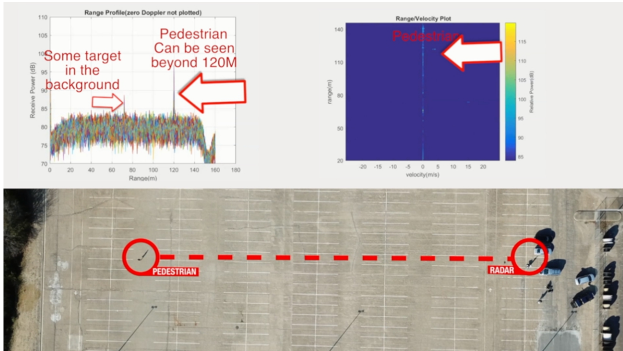
图 30. Range Profile (top left), and Doppler-Range Plot of a Pedestrian Jogging Away From Radar at 120 Meters Range
