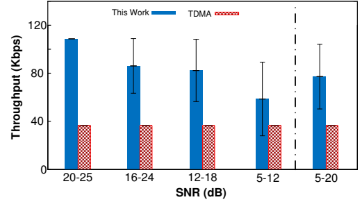
Fig. 11—Channel Quality versus Throughput for Distributed Rate Adaptation. AirShare enables distributed rate adaptation for wireless sensors.
