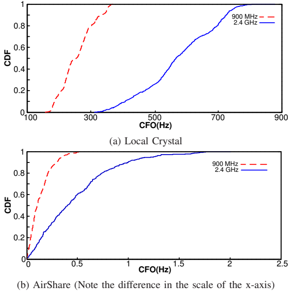
Fig. 5—CFO between pairs of nodes at carrier frequencies of 2.4 GHz and 900 MHz: (a) Independent clocks and (b) AirShare. Comparing (a) and (b), AirShare reduces the CFO by multiple orders of magnitude.
