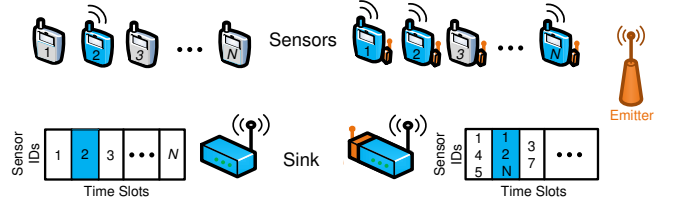
Fig. 10—Traditional Sensor Networks (left) vs. Distributed Rate Adaptation (right). A blue node indicates an active sensor. With traditional sensor networks, only one sensor transmits at a time. In contrast, AirShare-equipped sensors perform distributed rate adaptation by transmitting simultaneously. This enables decoding data from multiple sensors in a single joint transmission, and consumes significantly fewer than N slots to transmit data from all N sensors.
