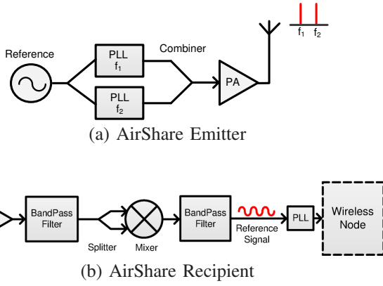
Fig. 3— AirShare’s System Architecture. The AirShare emitter includes two PLLs to generate two single tones separated by the desired frequency. The AirShare recipient mixes the received AirShare signal with itself and extracts the reference clock using a band pass filter.
