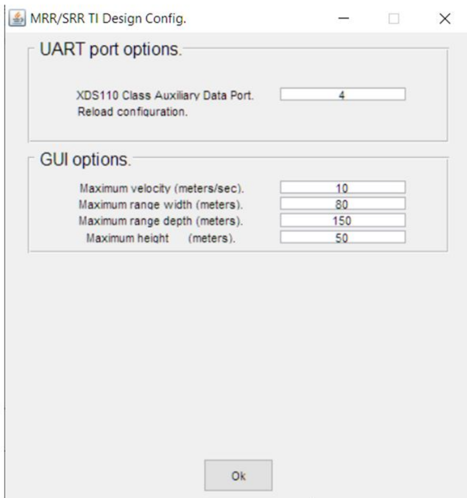
Figure 11. GUI Configuration
