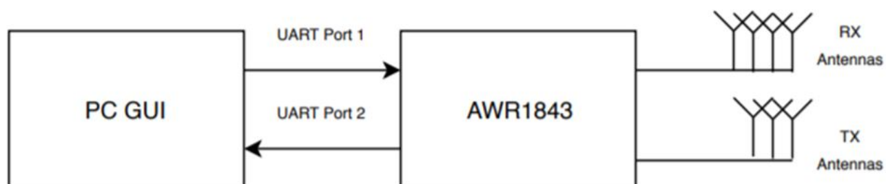
Figure 1. BSD, LCA, TJA System Block Diagram
