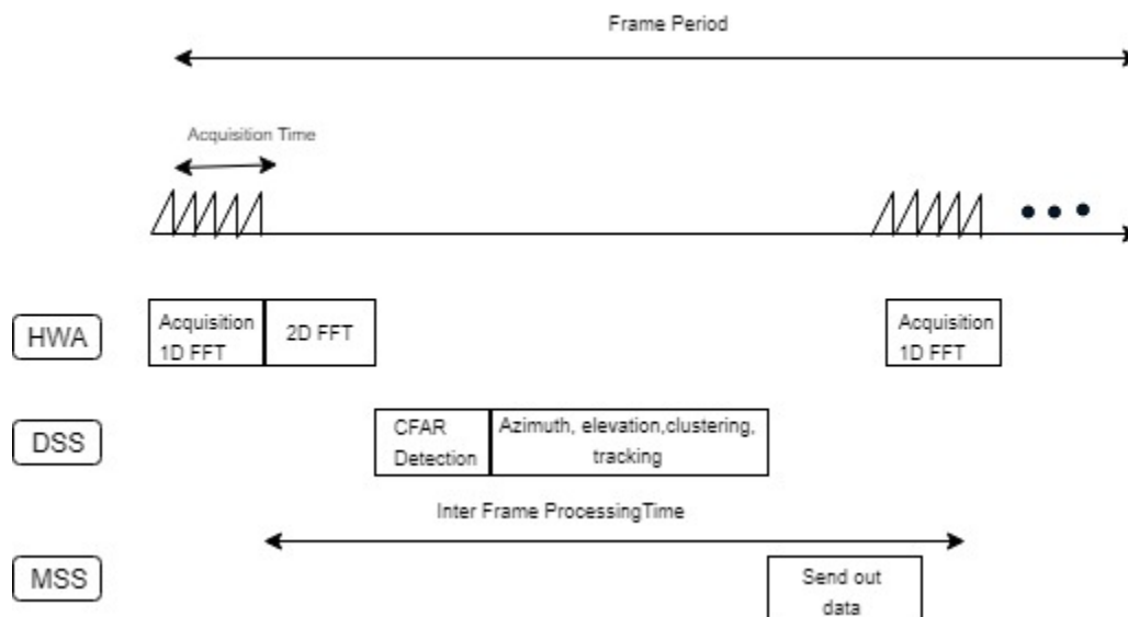
Figure 6. Top Level Data Path Timing
