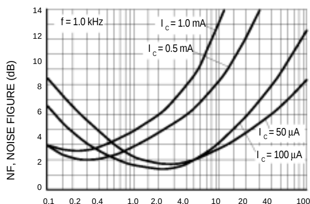
R_g , SOURCE RESISTANCE (kΩ) Figure 8. Noise Figure
