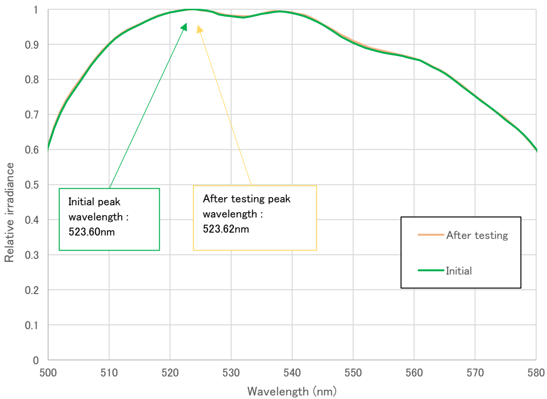
Graph3; Green LED spectrum (detail)
