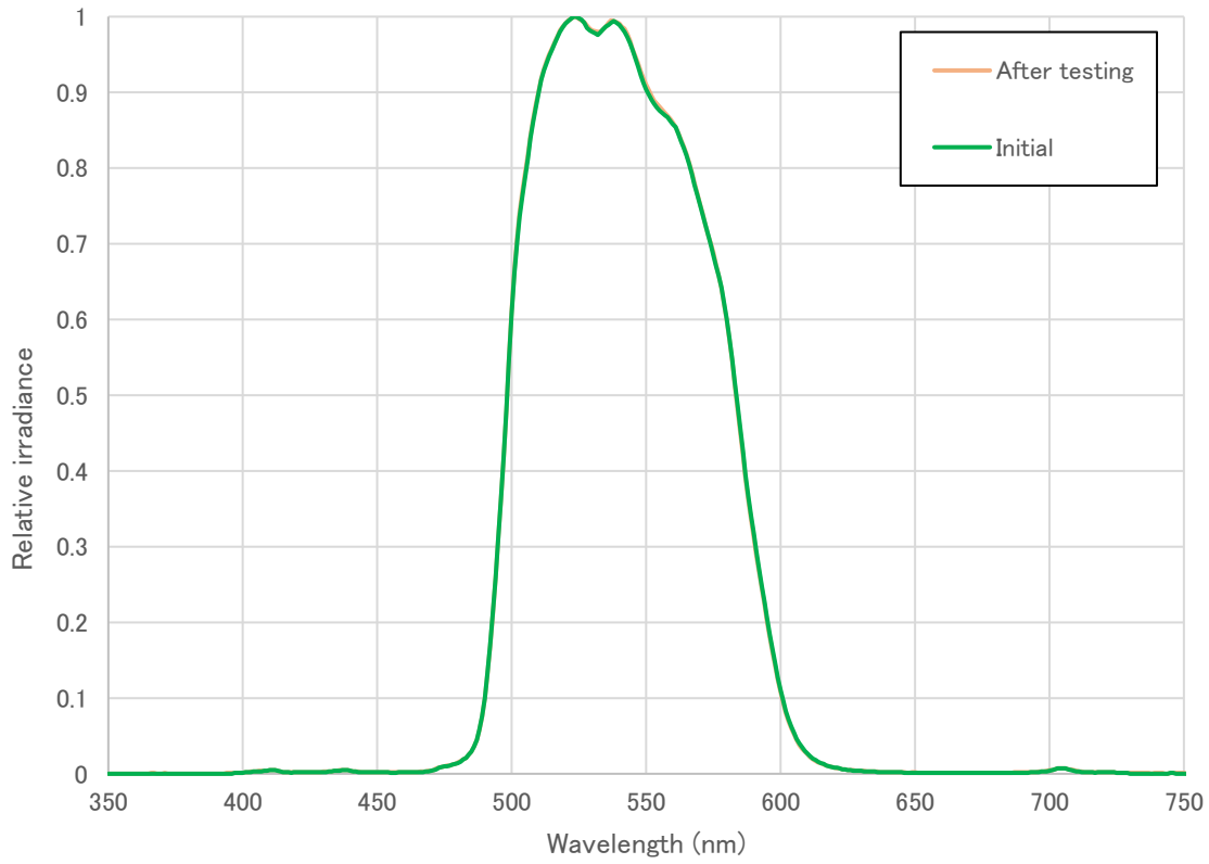
Graph2; Green LED spectrum
