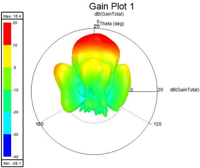
3D- Gain plot @ 60GHz
