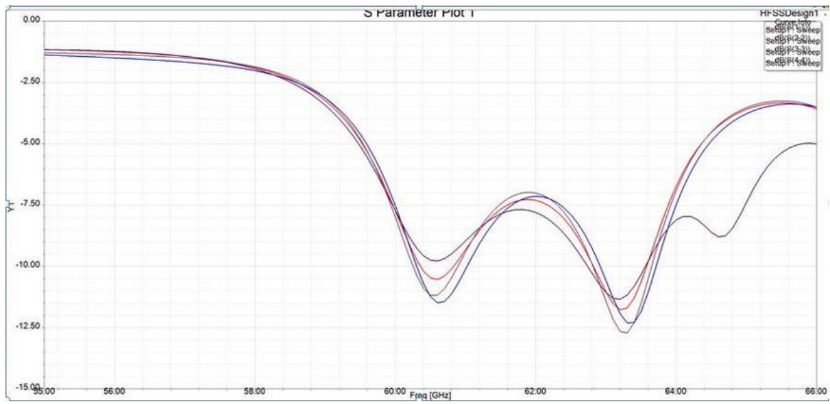
Return loss/S-Parameter plot of all 4 Rx antennas from 59-66GHz shared by TI in the forum
