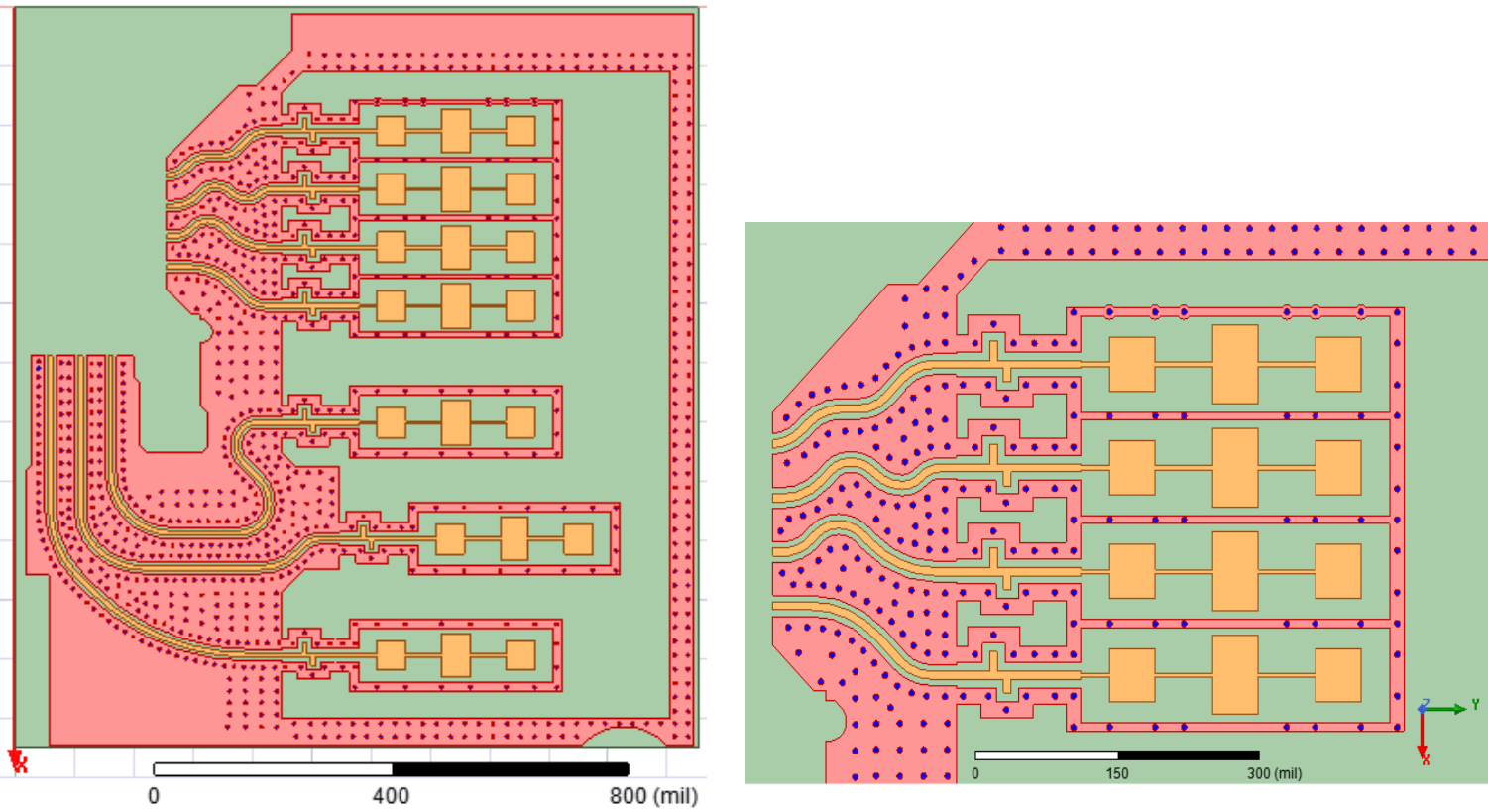
Top View of the board with on board antennas
