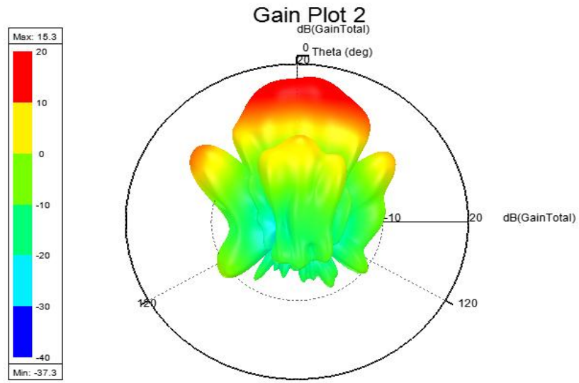
3D- Gain plot @ 61GHz
