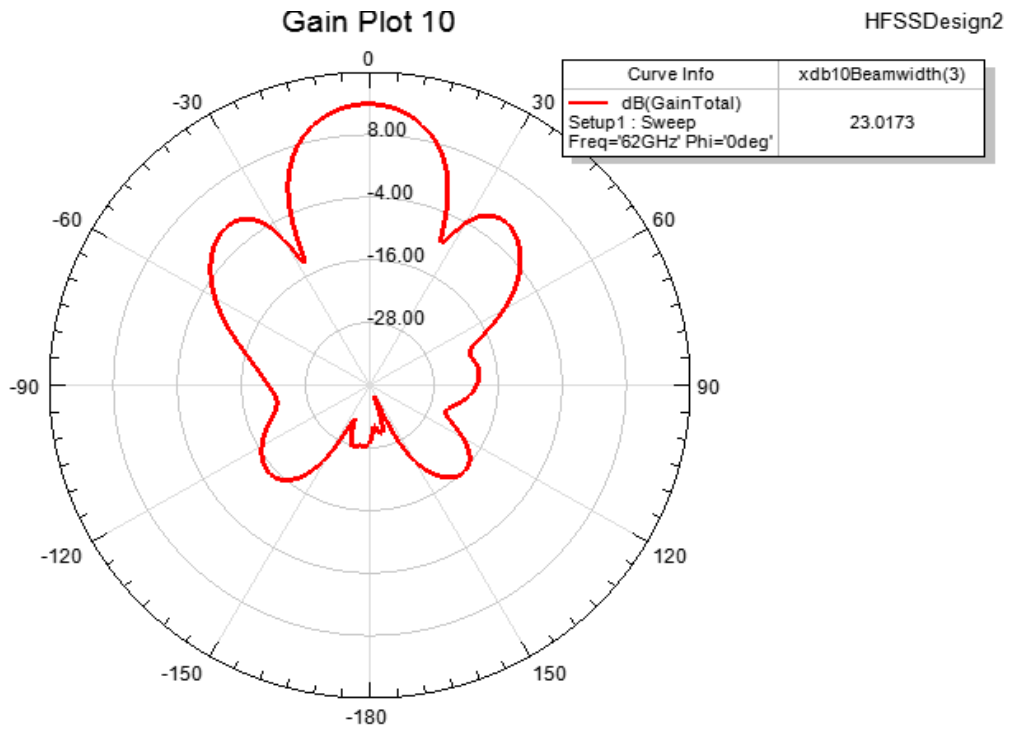
Elevation 2D Radiation plot @ 62GHz
