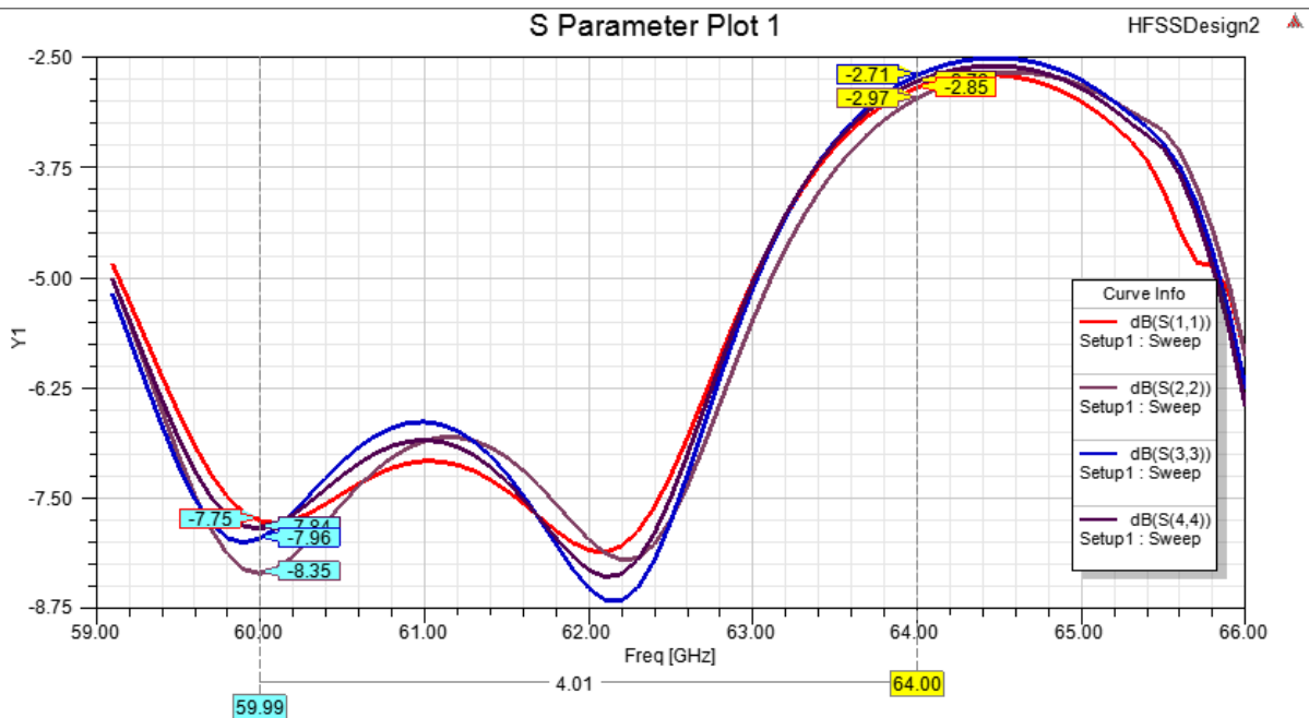
Return loss/S-parameter plot of all 4 Rx antennas from 59-66GHz as obtained by our simulations
