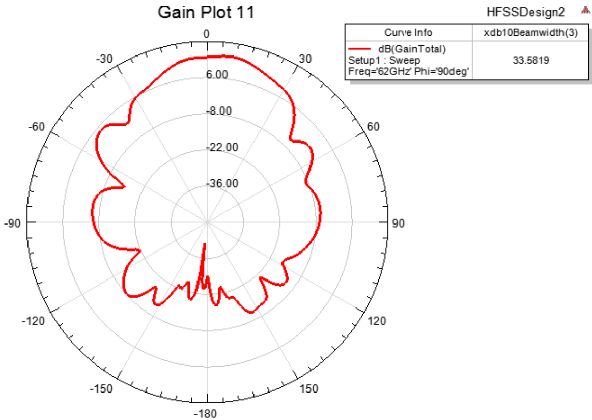
Azimuth 2D Radiation plot @ 62GHz
