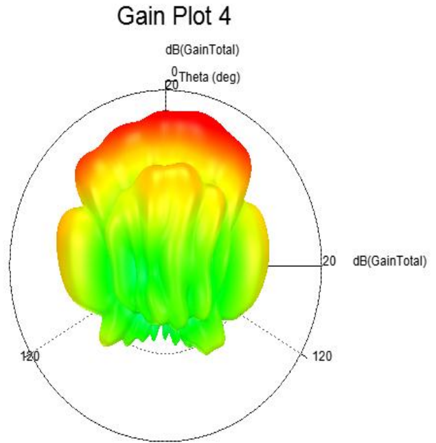
3D- Gain plot @ 63GHz
