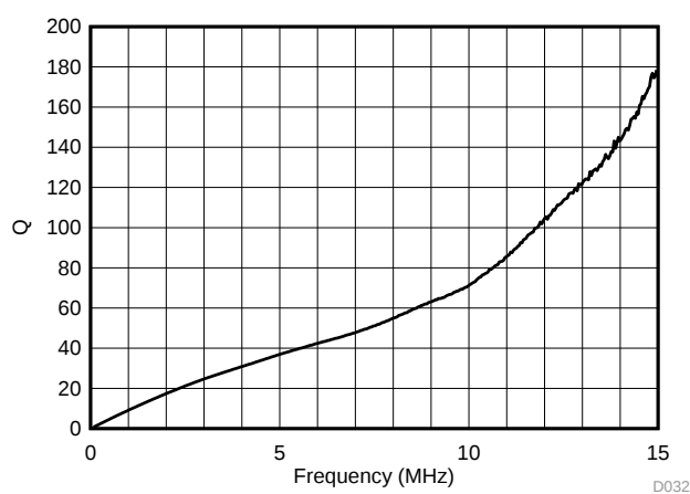
Figure 33. Coil Q: Q vs. Frequency
