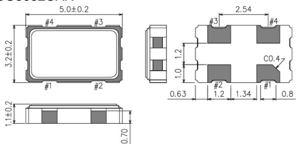
SG5032CAN
