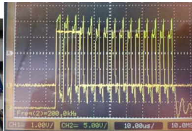
Start + Transmitter 15 excitation cycles
