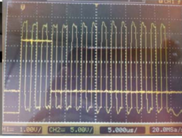
Start + Transmitter 15 excitation cycles
